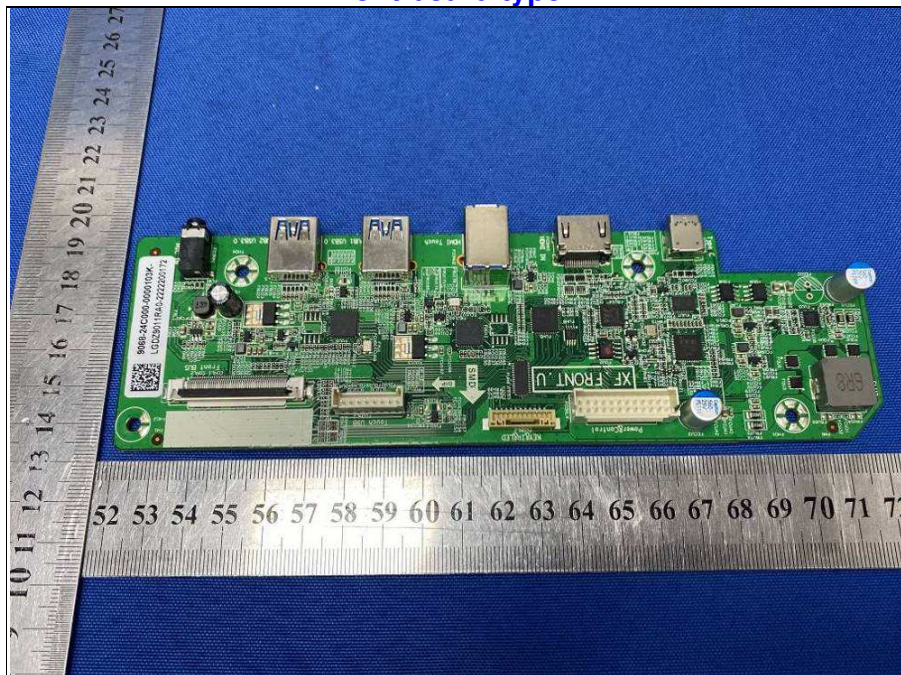
Front board type A
