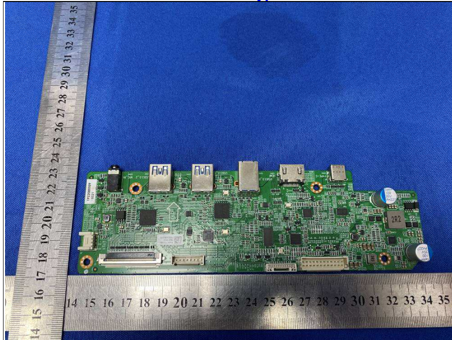
Front board type B
