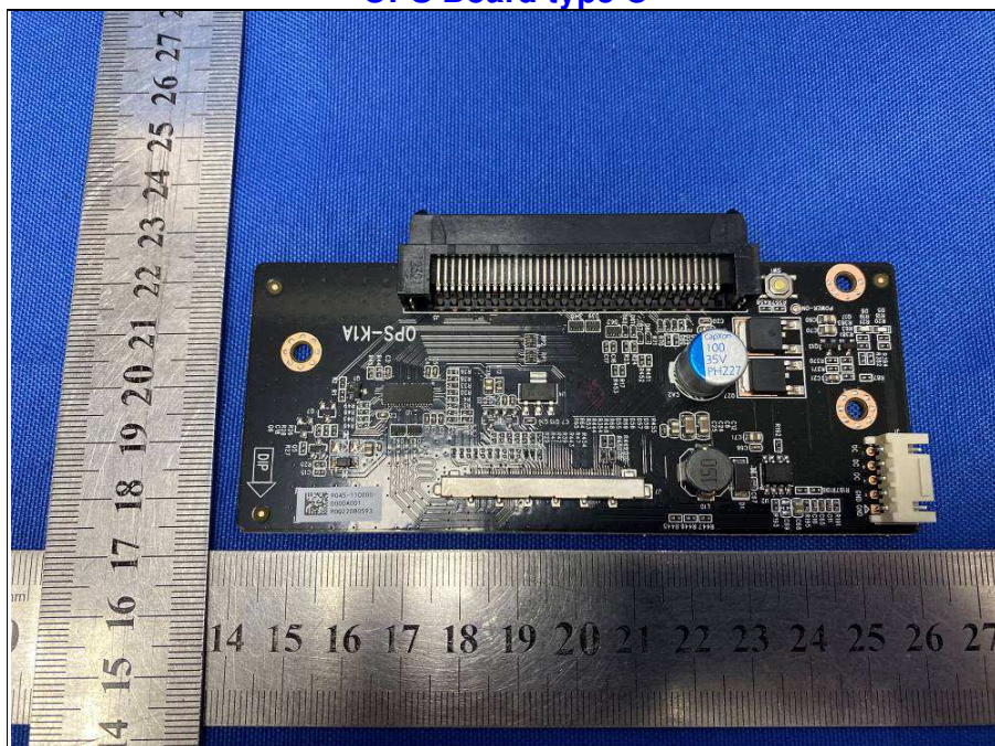
OPS Board type C
