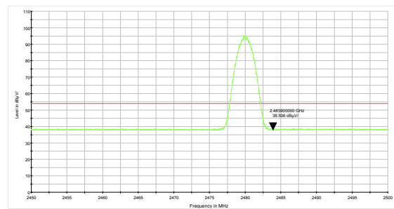
3DH5-Channel 78: Average
