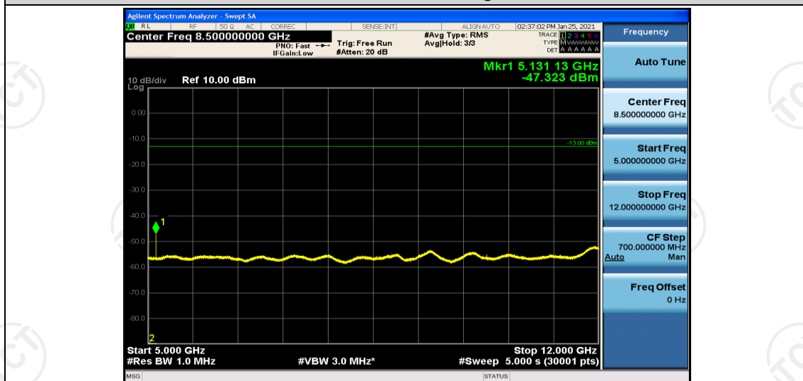
Band66-5MHz-QPSK-131997-1RB#0-Range6:12000~26500MHz
