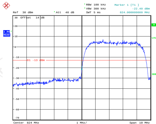
Lower Band Edge Plot on Channel 4132
