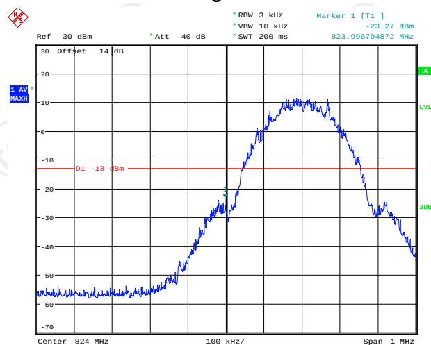
Lower Band Edge Plot on Channel 128
