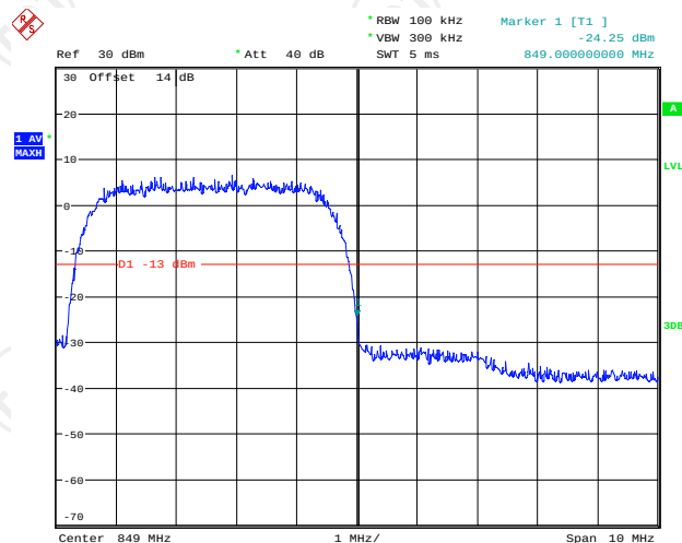
Higher Band Edge Plot on Channel 4233
