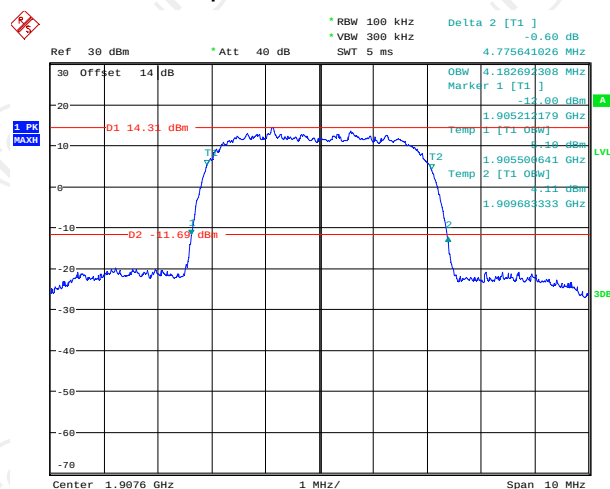
26dB&99% Occupied Bandwidth Plot on Channel 9538
