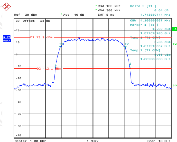
26dB&99% Occupied Bandwidth Plot on Channel 9400
