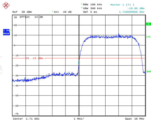
Lower Band Edge Plot on Channel 1312
