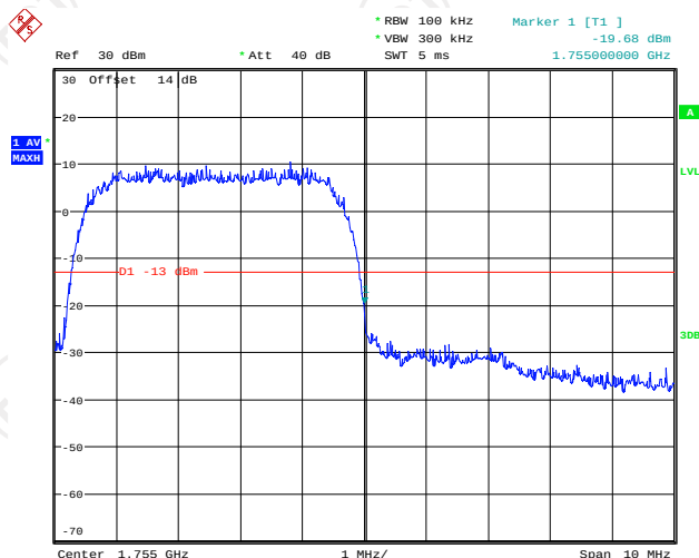
Higher Band Edge Plot on Channel 1513
