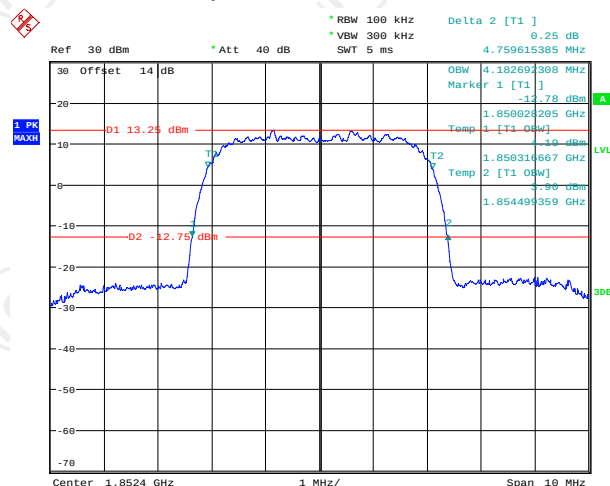
26dB&99% Occupied Bandwidth Plot on Channel 9262
