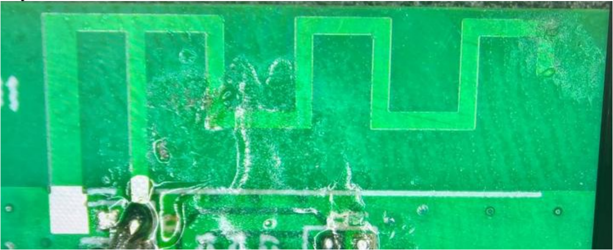
Physical antenna and dimensions
