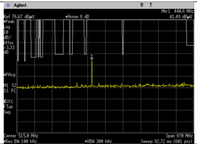
Low Ch_2402MHz_2MBit_15.209_30-1000MHz_Peak
