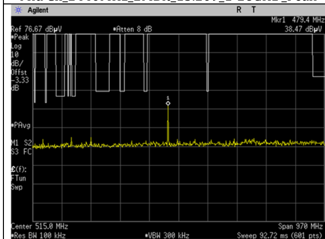
Mid Ch_2440MHz_2MBit_15.209_30-1000MHz_Peak
