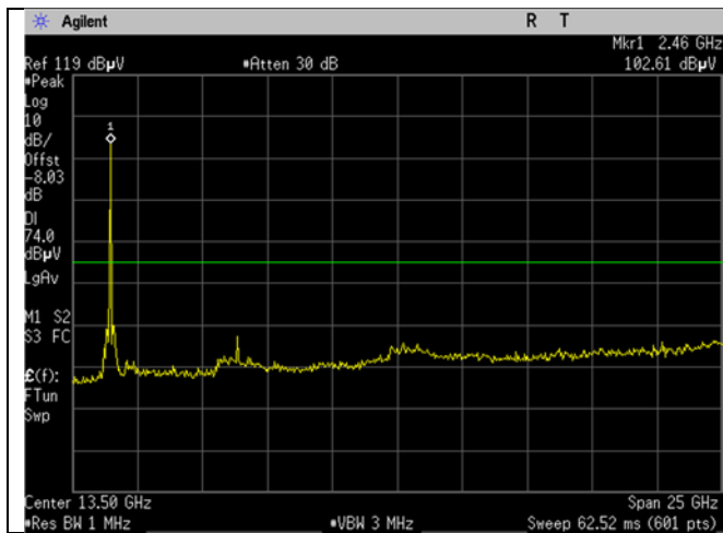
Mid Ch_2440MHz_2MBit_15.209_1-26GHz_Peak
