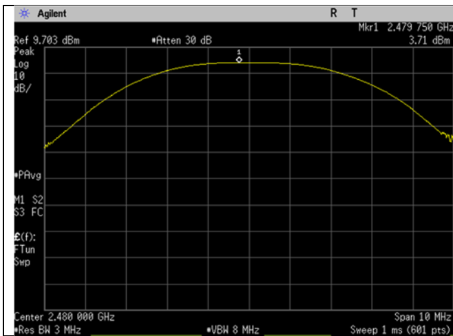
High Ch_2480MHz_2MBit_Output Power
