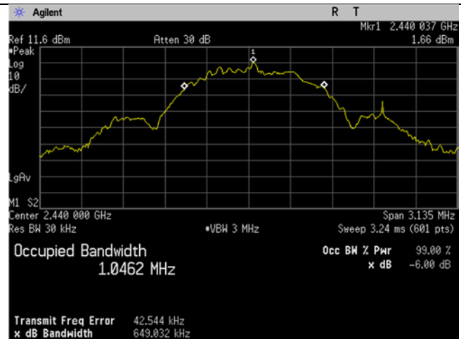
Mid Ch_2440MHz_1MBit_Occupied Bandwidth_99 percent_
