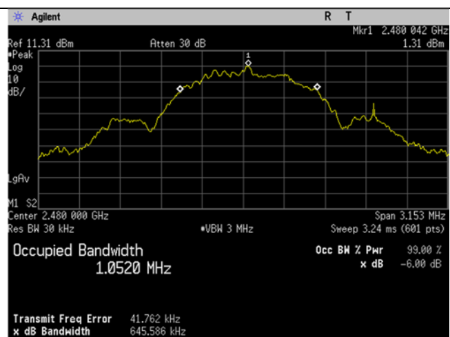
High Ch_2480MHz_1MBit_Occupied Bandwidth_99 percent_
