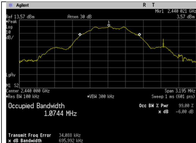
Mid Ch_2440MHz_1MBit_Occupied Bandwidth_6dB_
