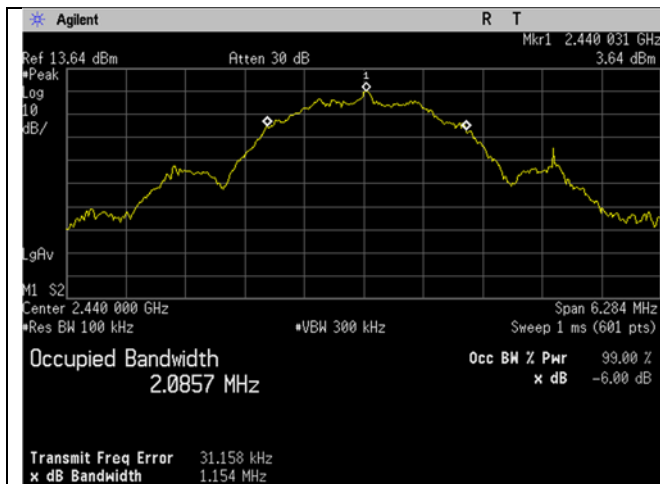
Mid Ch_2440MHz_2MBit_Occupied Bandwidth_-6dB
