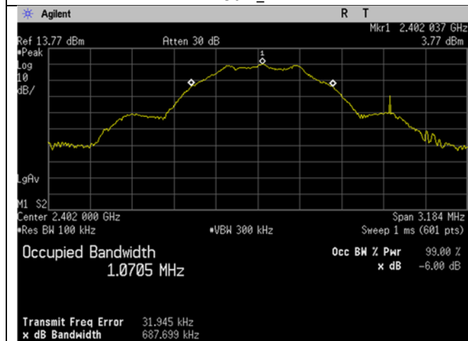
Low Ch_2402MHz_1MBit_Occupied Bandwidth_-6dB_
