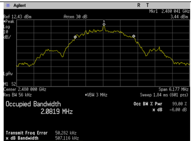
High Ch_2480MHz_2MBit_Occupied Bandwidth_99 percent
