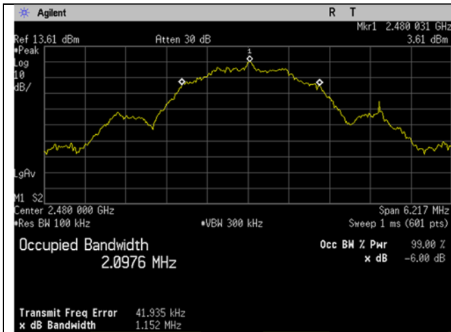
High Ch_2480MHz_2MBit_Occupied Bandwidth_6dB
