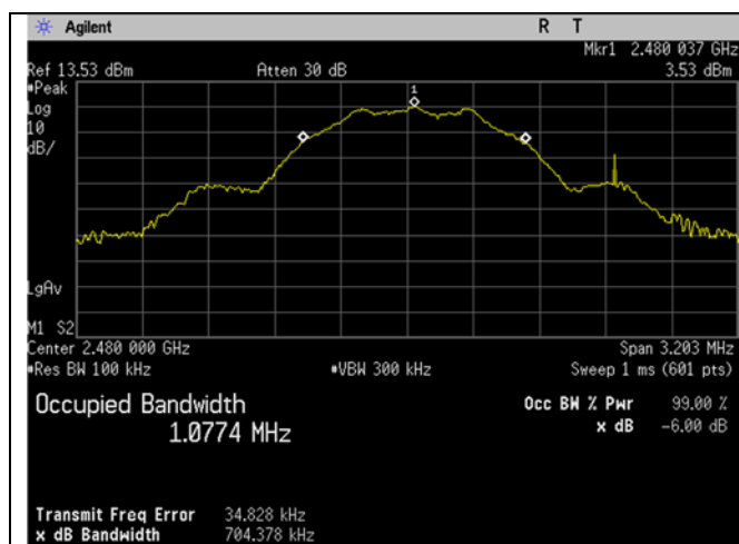
High Ch_2480MHz_1MBit_Occupied Bandwidth_-6dB_
