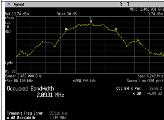
Low Ch_2402MHz_2MBit_Occupied Bandwidth_6dB
