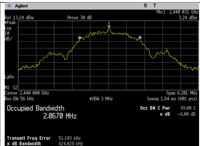
Mid Ch_2440MHz_2MBit_Occupied Bandwidth_99 percent
