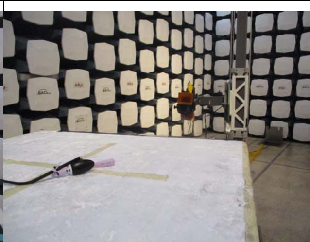
18-26.5GHz Rear View
