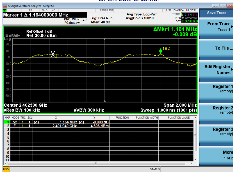
Test plots GFSK Low Channel
