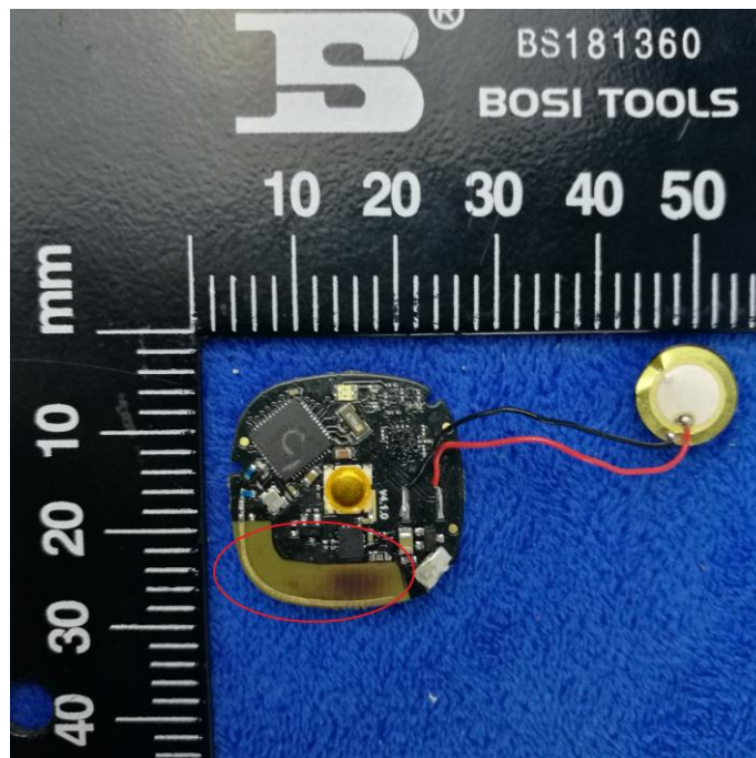
Antenna View
