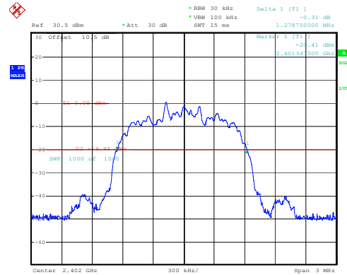
2DH1_Low 1.279MHz
