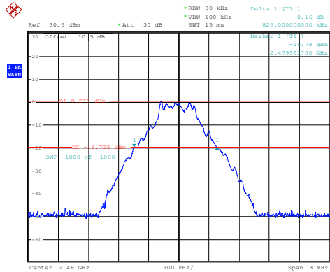
DH1_High 0.825MHz
