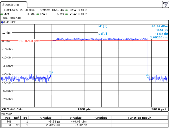
3DH5_Hopping 2.903ms
