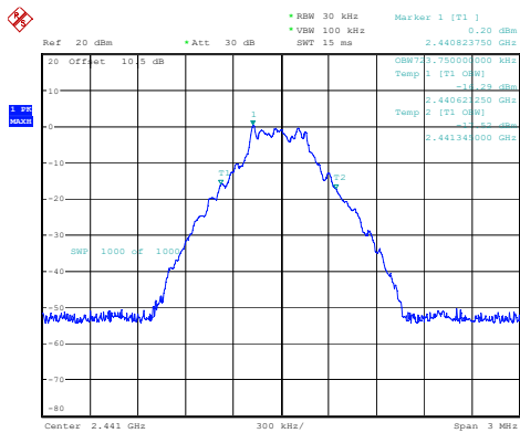
DH1_Middle 0.724MHz
