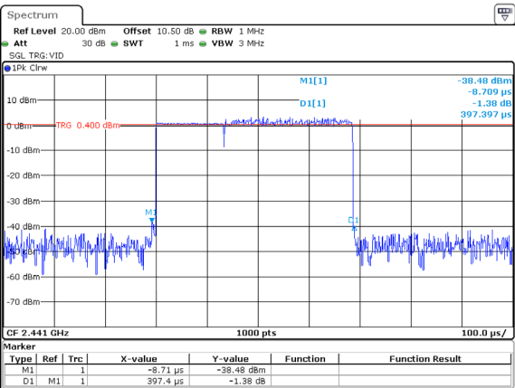
3DH1_Hopping 0.397ms
