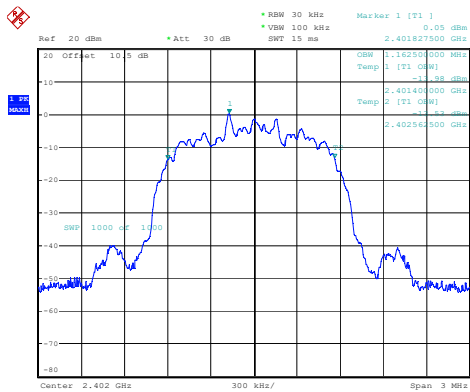
2DH1_Low 1.163MHz
