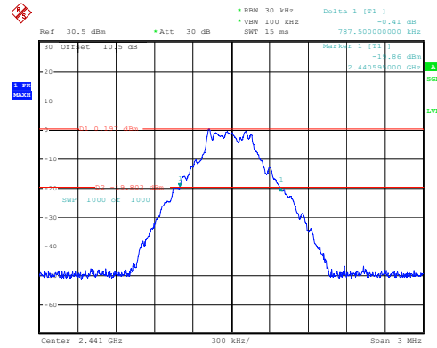
DH1_Middle 0.788MHz
