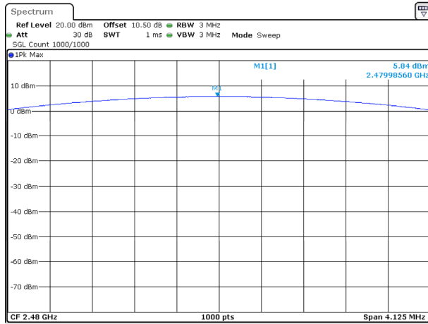
DH1_High
