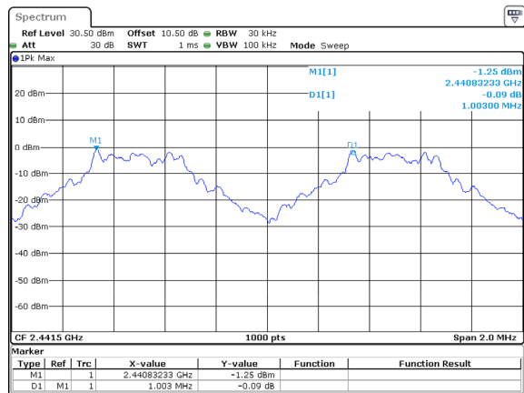
DH1_Middle 1.003MHz
