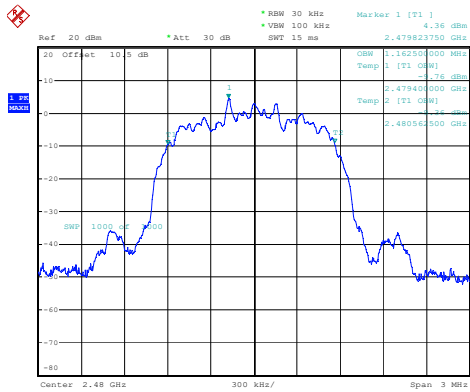
2DH1_High 1.163MHz
