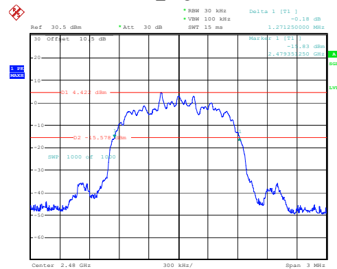
2DH1_High 1.271MHz
