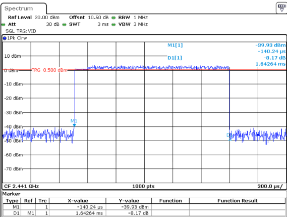
3DH3_Hopping 1.643ms
