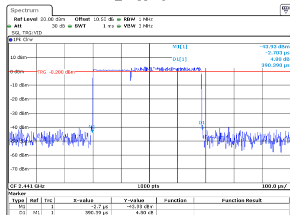
2DH1_Hopping 0.390ms
