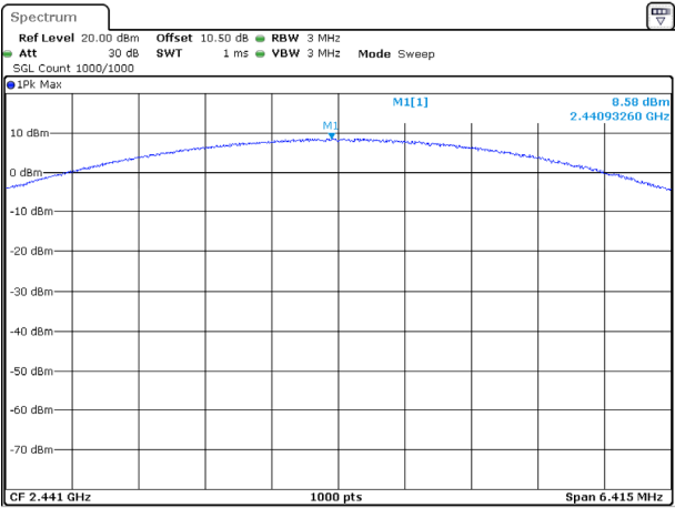
3DH1_Middle
