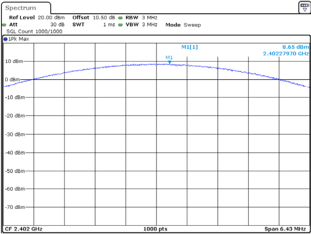
3DH1_Low
