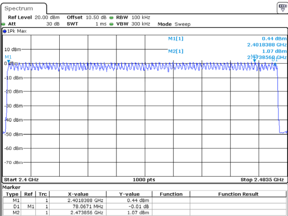
2DH1_Hopping 79
