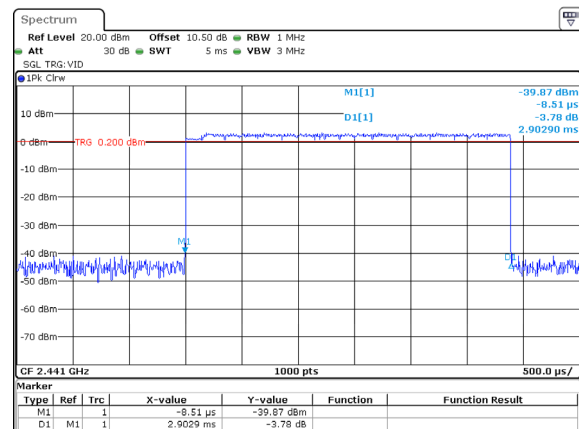
2DH5_Hopping 2.903ms
