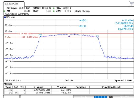
802.11n40_2437MHz_Chain 0
