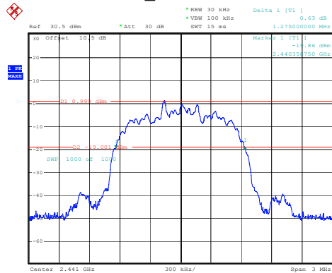
2DH1_Middle 1.275MHz
