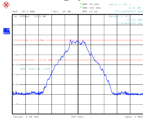
DH1_High 0.776MHz
