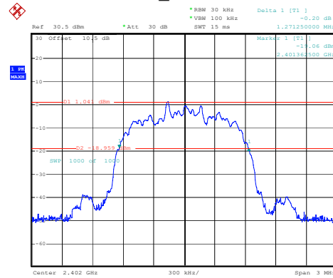
2DH1_Low 1.271MHz
