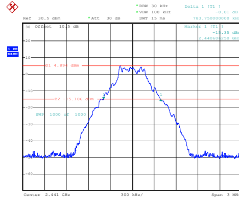
DH1_Middle 0.784MHz
