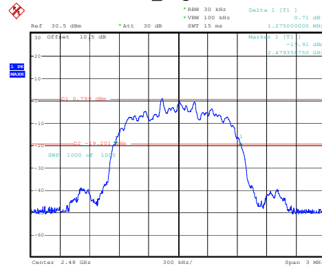
2DH1_High 1.275MHz
