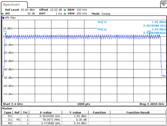
3DH1_Hopping 79
