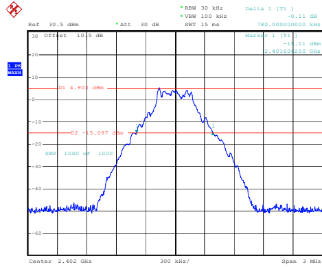
DH1_Low 0.780MHz
