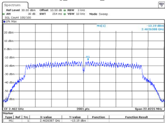
802.11g_2462MHz_Chain 1
