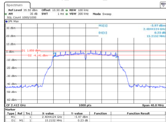
802.11g_2412MHz_Chain 1
