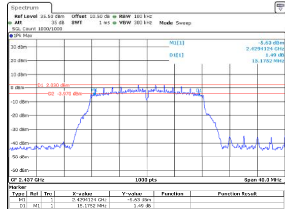
802.11g_2437MHz_Chain 0
