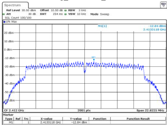
802.11g_2412MHz_Chain 1
