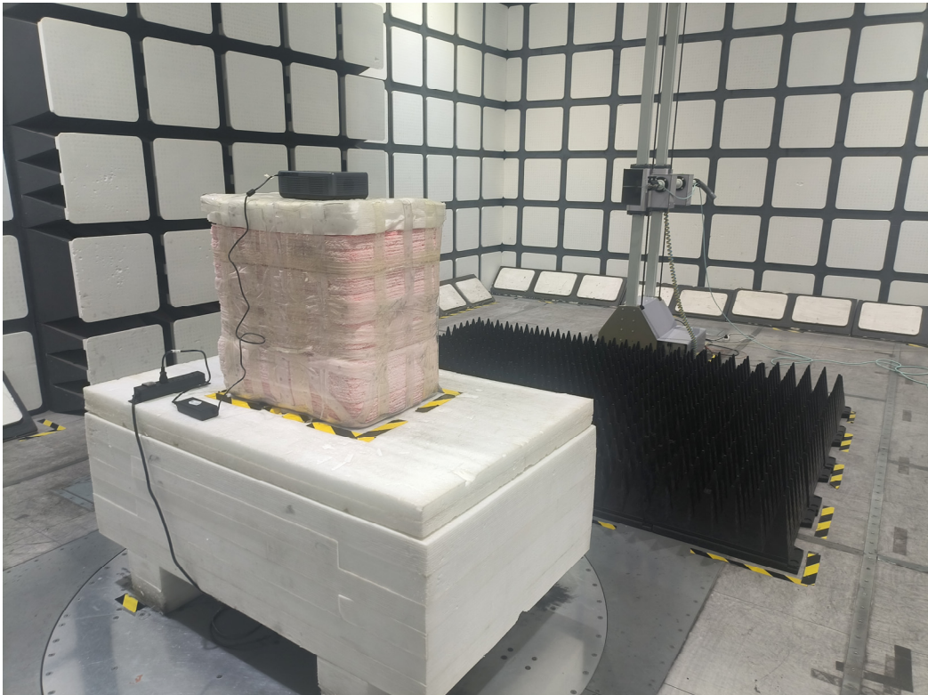
Radiated Emissions View (1-18 GHz)
