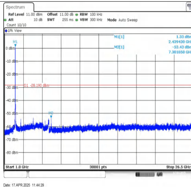
11N40SISO-Ant1-2437-1000~26500-PASS
