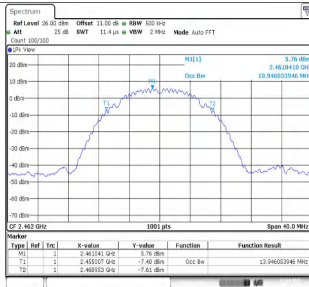
11B-Ant1-2462
