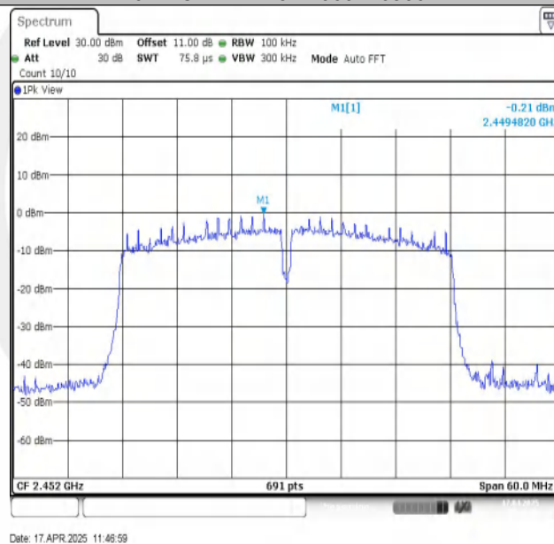
11N40SISO-Ant1-2452-0~Reference-PASS
