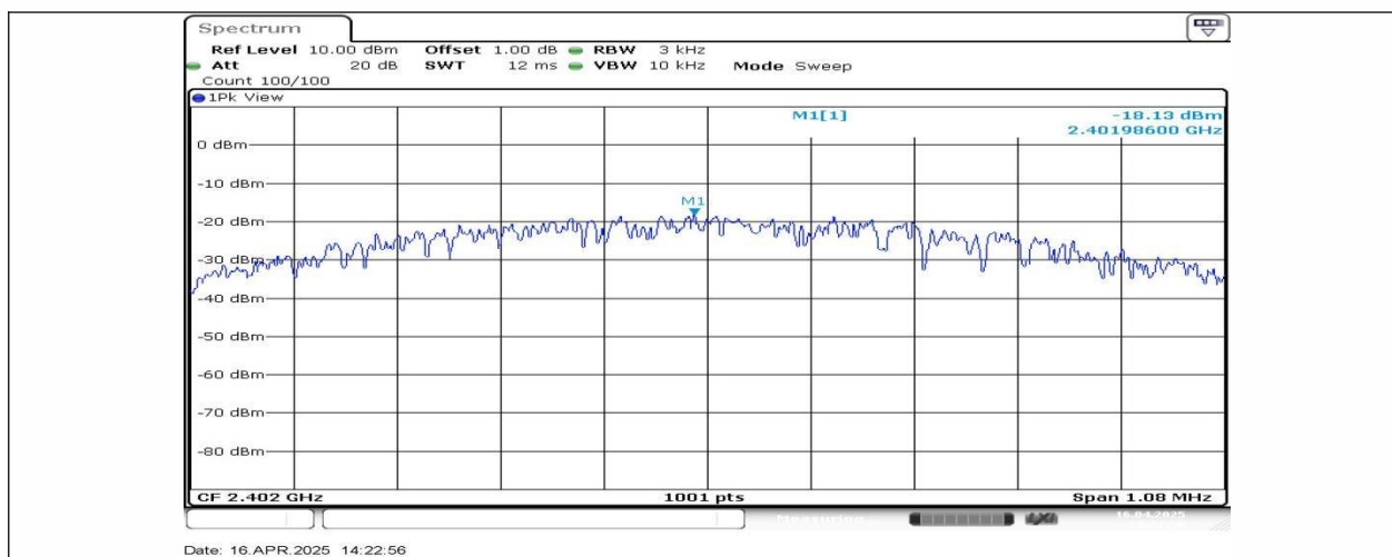
BLE_1M-Ant1-2402
