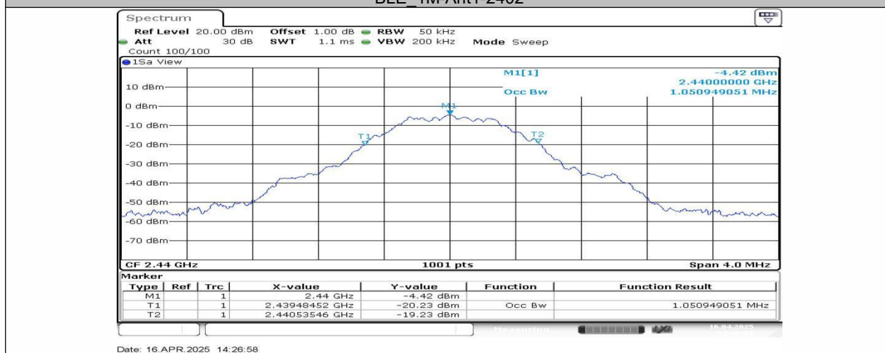
BLE_1M-Ant1-2440
