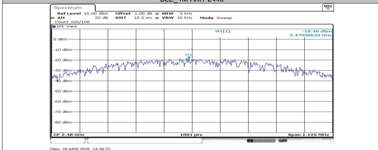
BLE_1M-Ant1-2480
