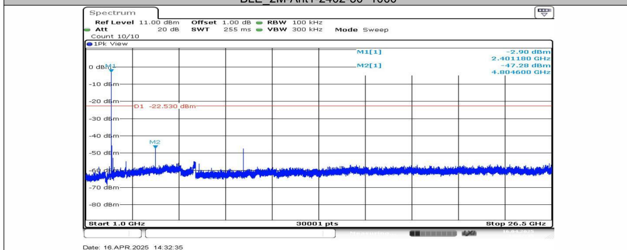
BLE_2M-Ant1-2402-1000~26500
