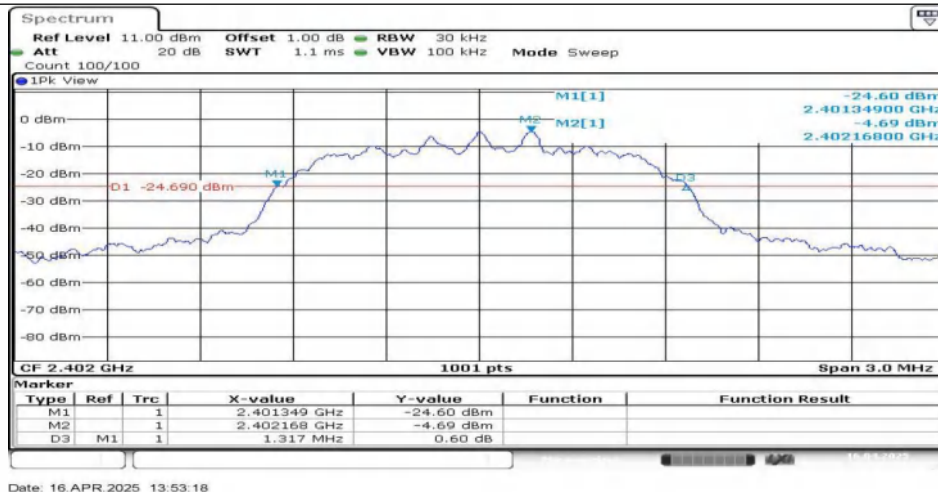
2DH5-Ant1-2402
