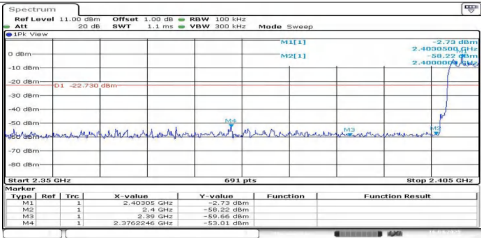
2DH5-Ant1-Hop_2402
