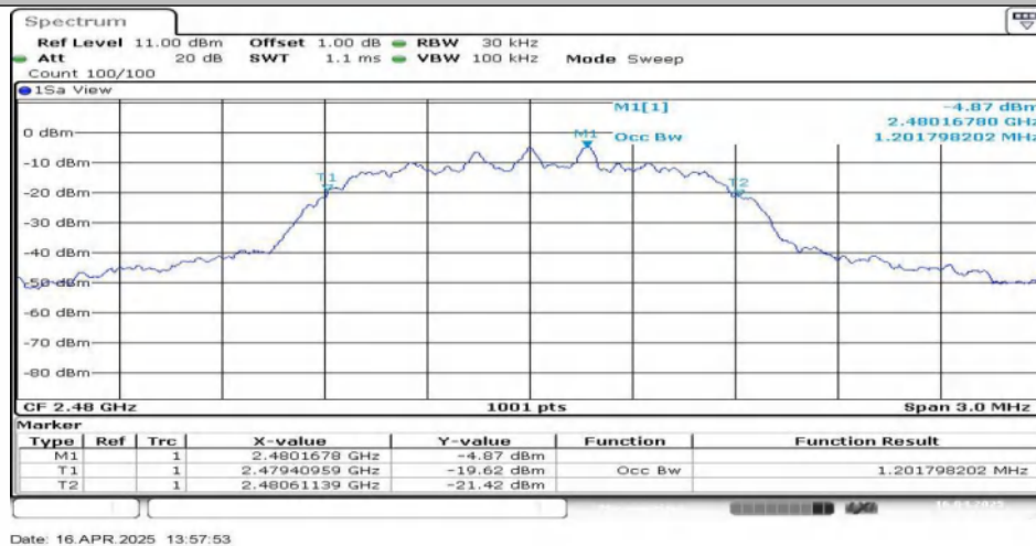
2DH5-Ant1-2480
