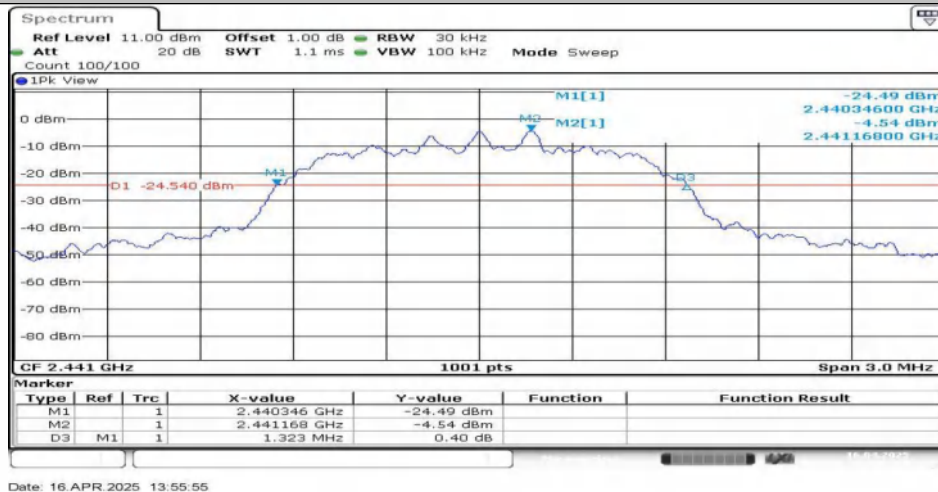
2DH5-Ant1-2441
