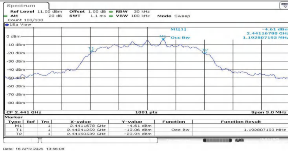
2DH5-Ant1-2441
