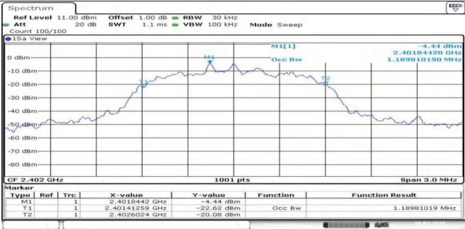
3DH5-Ant1-2402
