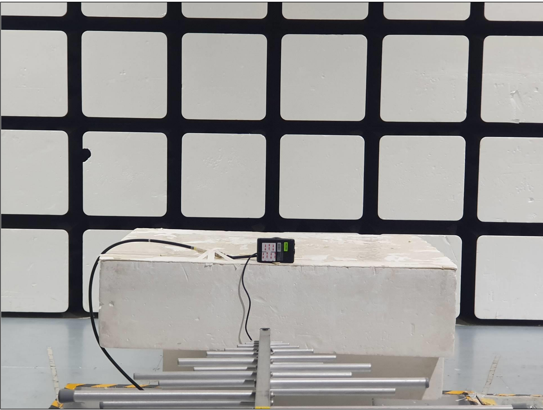
RE(Below 1 GHz)_Rear
