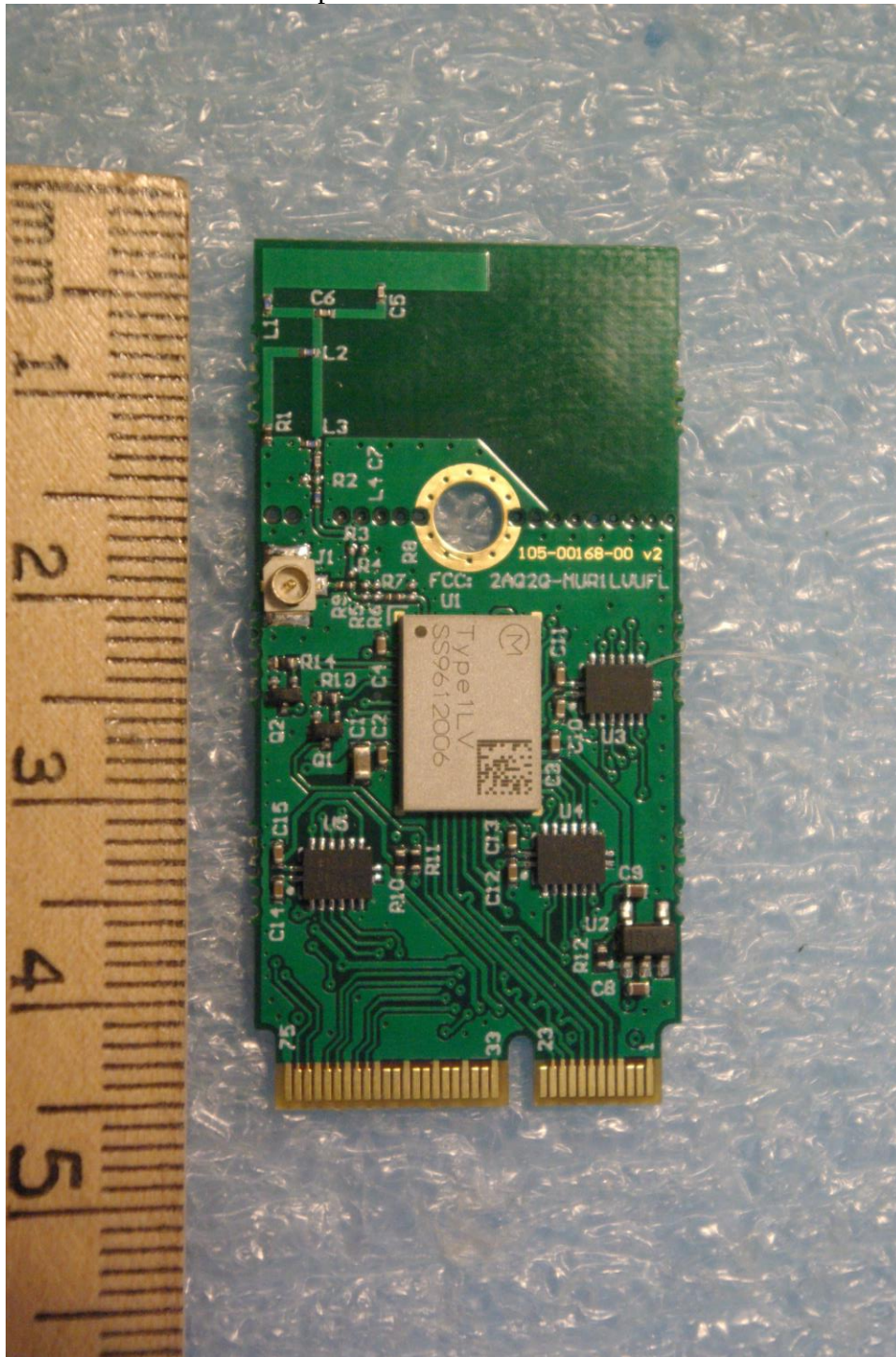
Module Placed on Development Circuit Board
