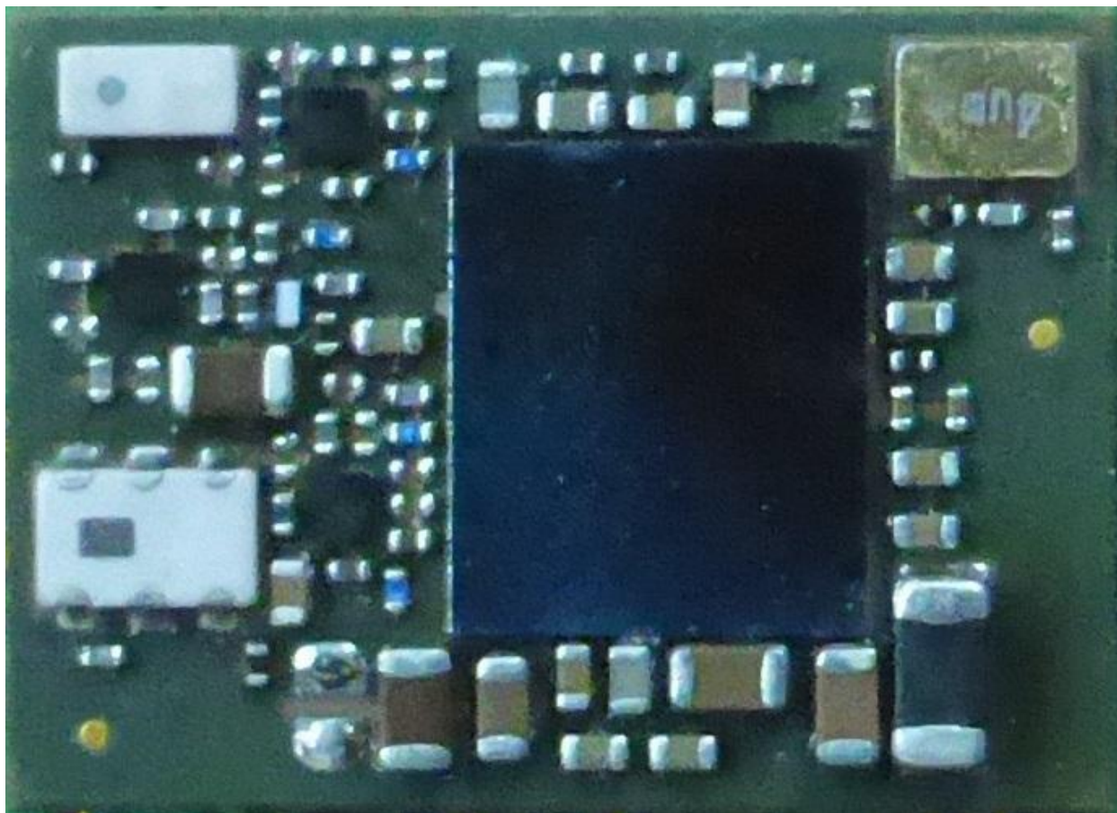
Module Only, cover removed
