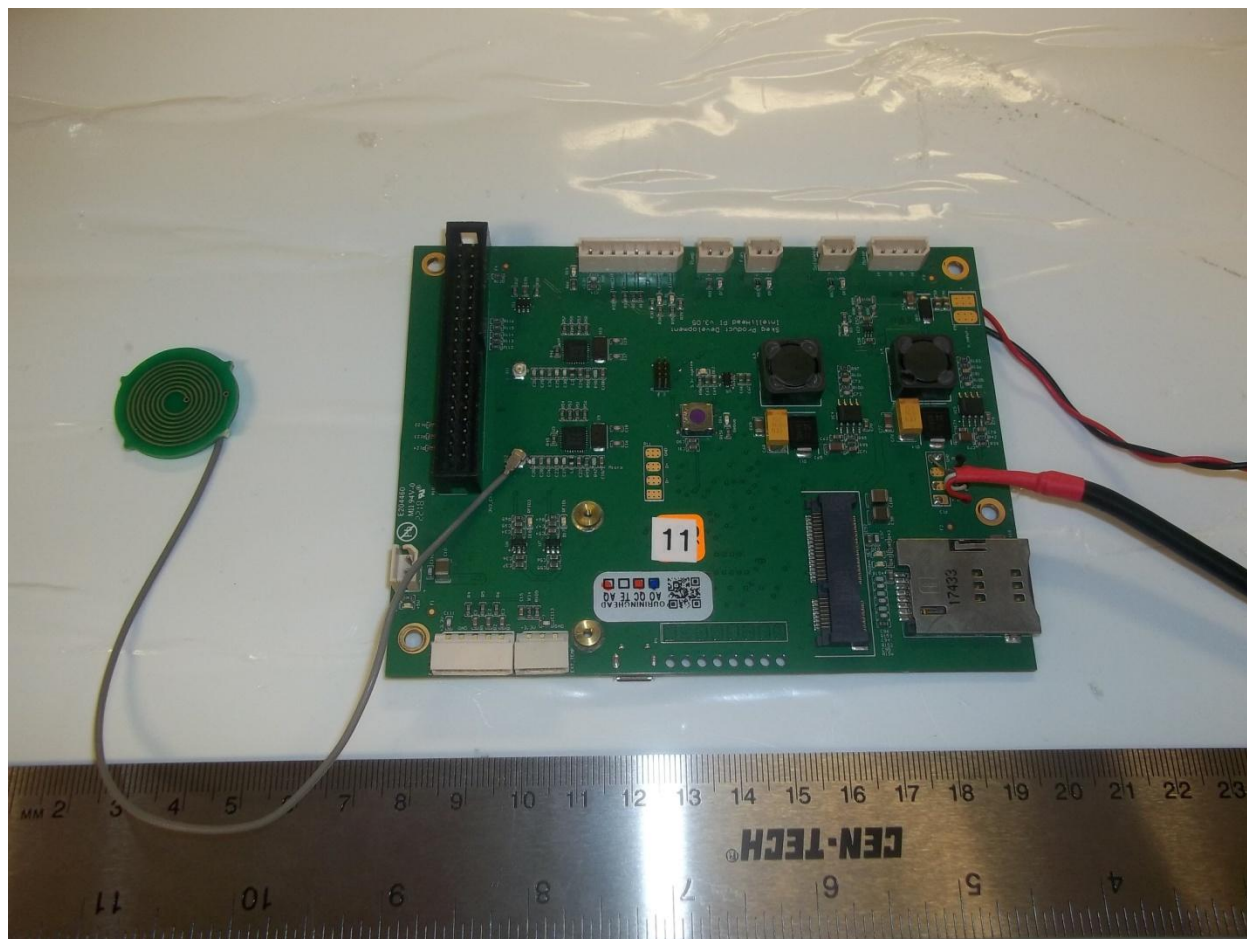
Figure 1. EUT, Radio Module board (Front Side)
