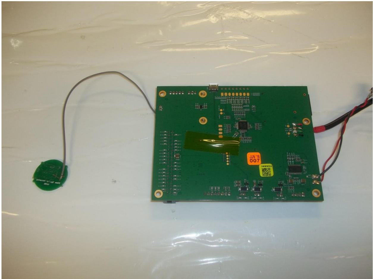
Figure 2. EUT, Radio Module board (Back Side)
