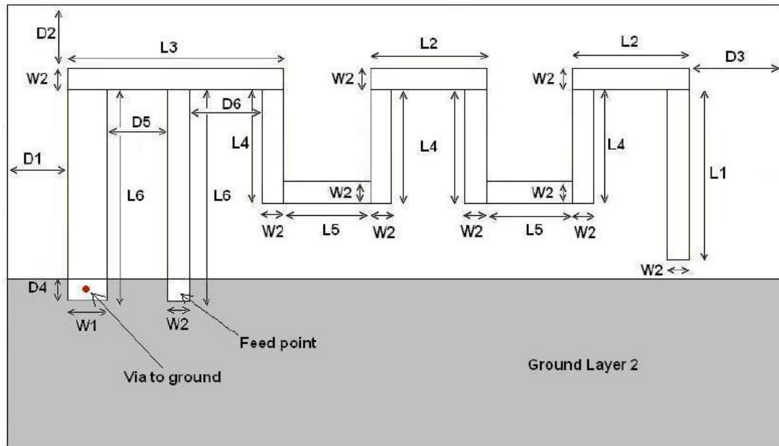
Figure 3: Antenna Dimensions
