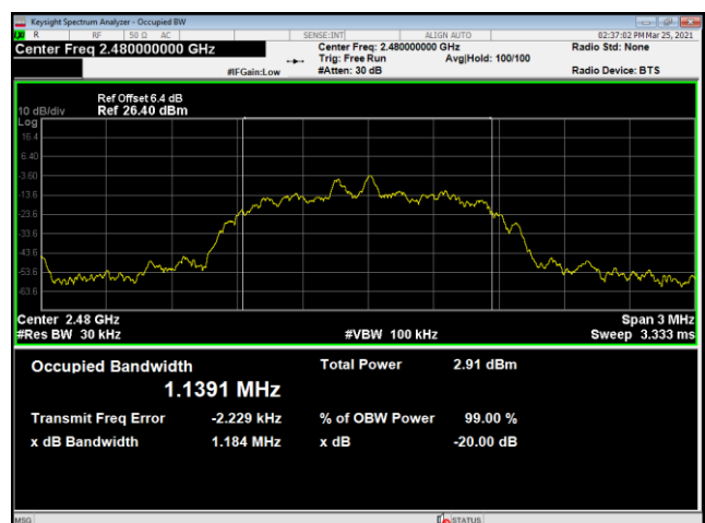
\pi/4 -DQPSK Highest channel
