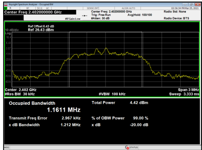
\pi/4 -DQPSK Lowest channel
