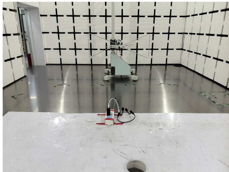
Radiated Emissions
