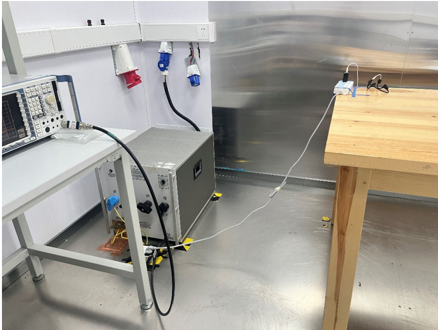
Conducted Emissions
