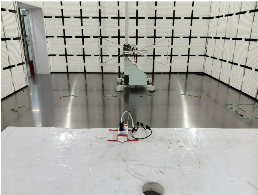
Radiated Emissions
