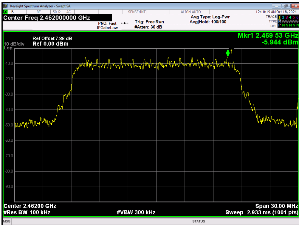
Tx. Spurious NVNT 802.11g 6Mbps 2462MHz Ant1 Emission
