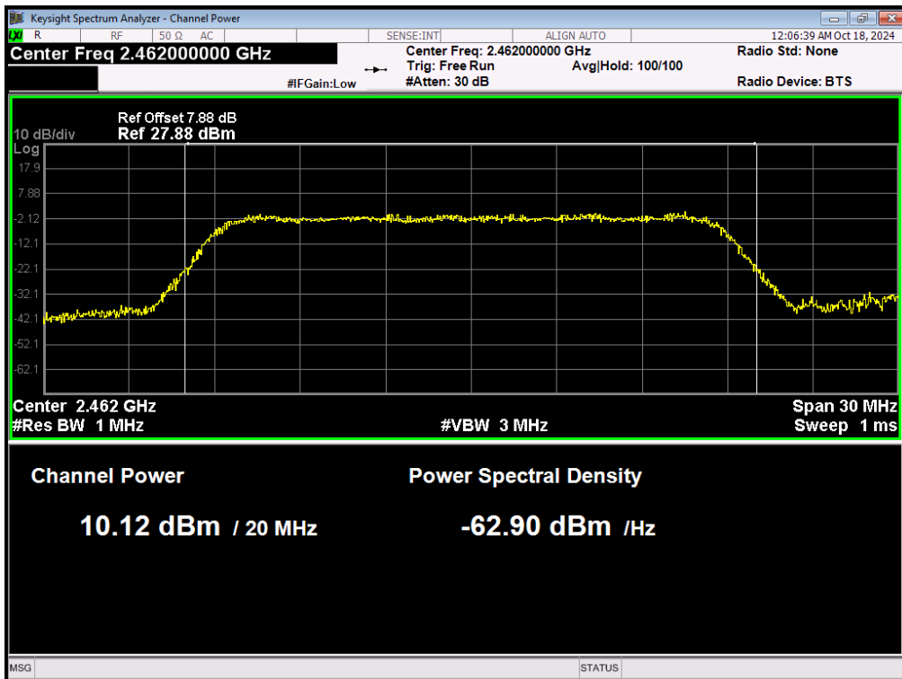
Power NVNT 802.11g 6Mbps 2462MHz Ant1
