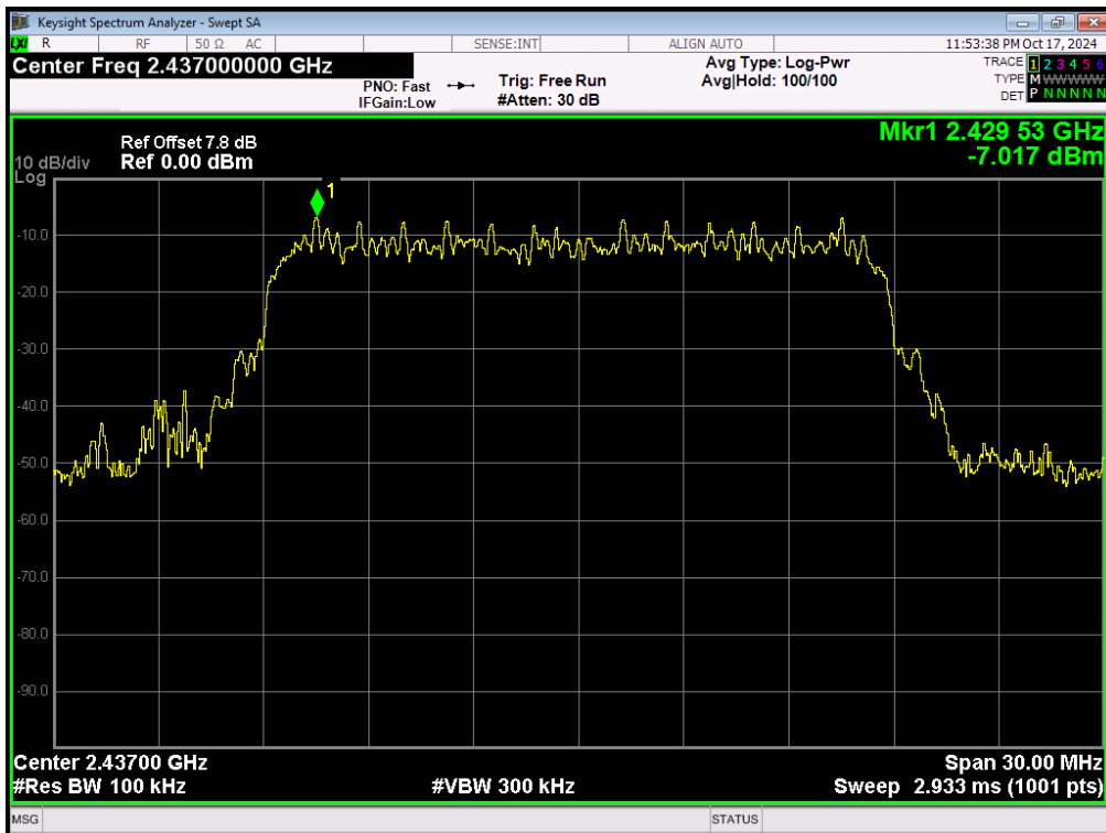
Tx. Spurious NVNT 802.11b 1Mbps 2437MHz Ant1 Emission
