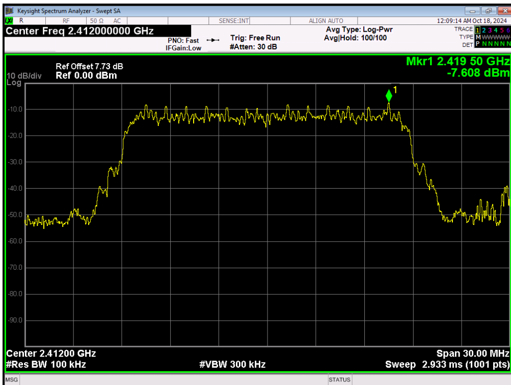
Tx. Spurious NVNT 802.11g 6Mbps 2412MHz Ant1 Ref
