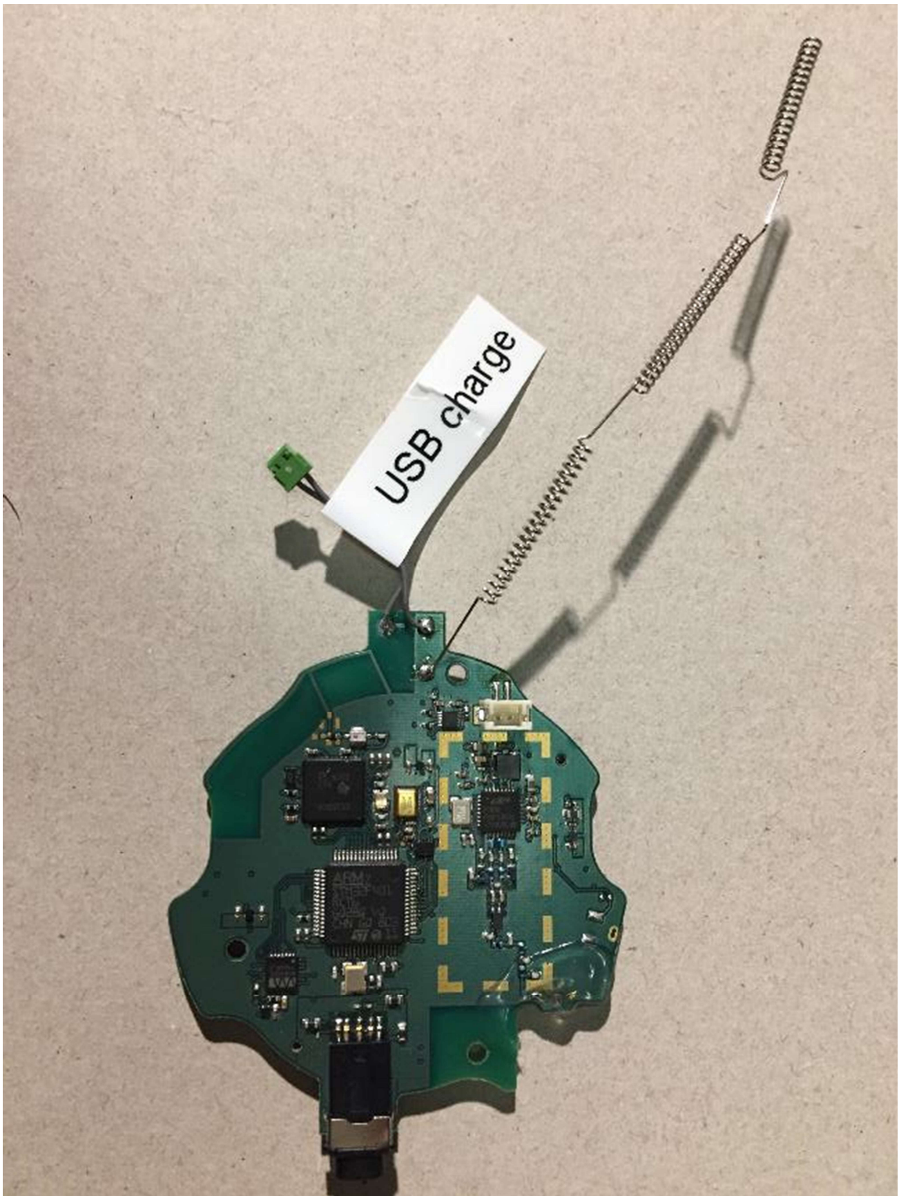
Side 1 of 2 (Shield removed. VHF antenna connected.)
