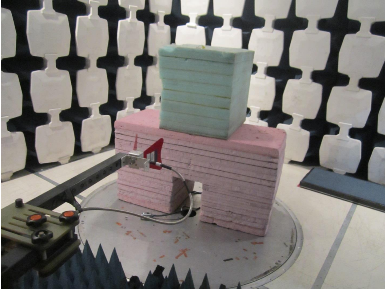
Preliminary 6-10GHz
