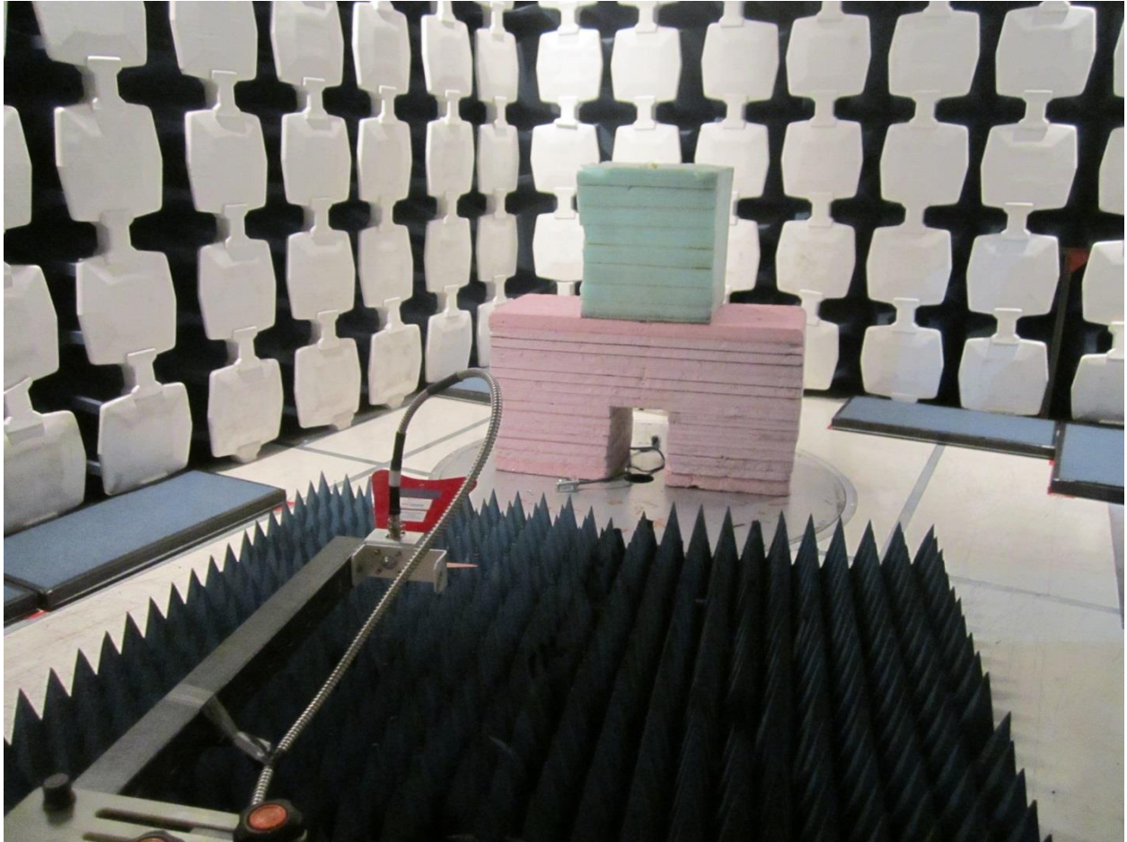
Preliminary 1-6GHz
