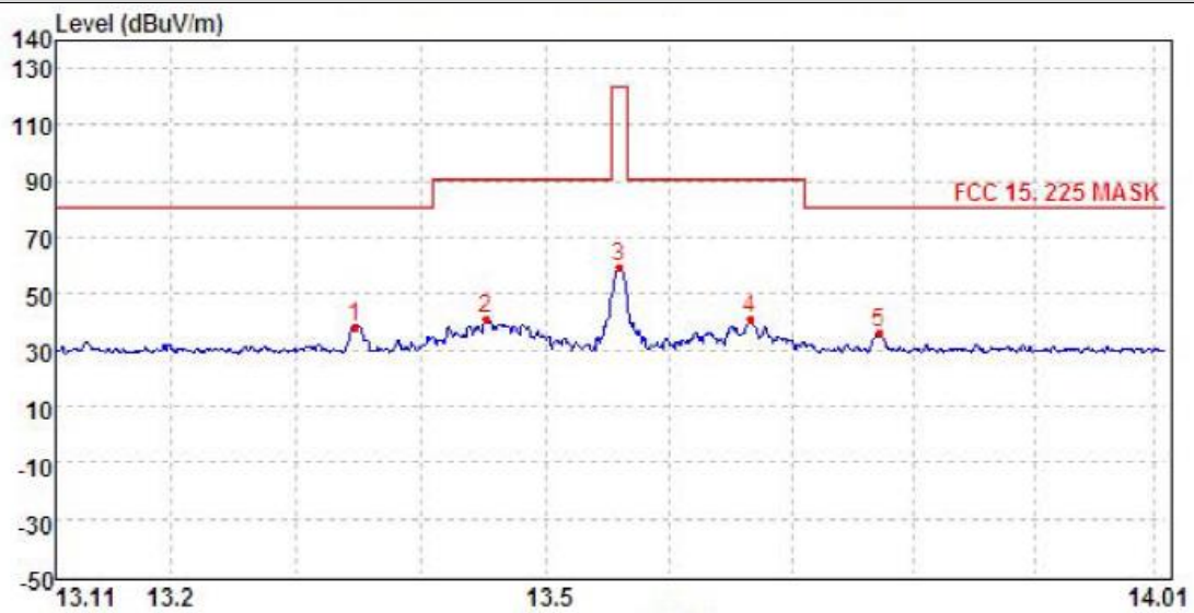
Field Strength of The Fundamental and Mask
