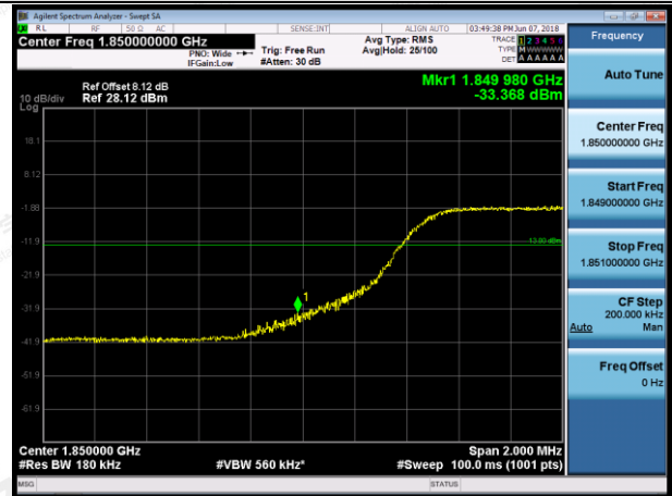
LCH_16QAM_50RB#0
