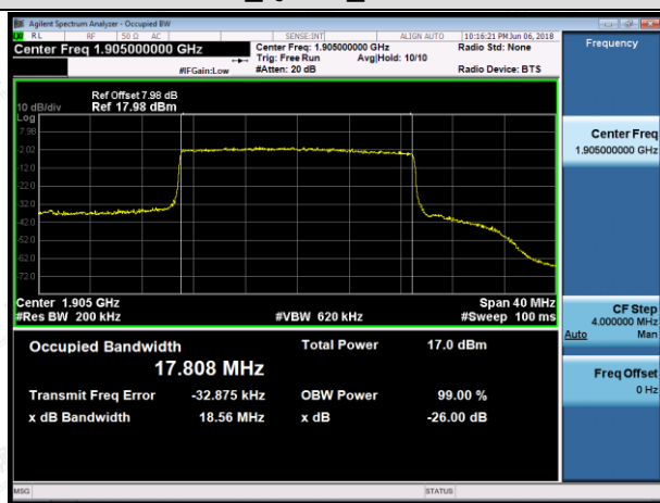
HCH_QPSK_100RB#0
