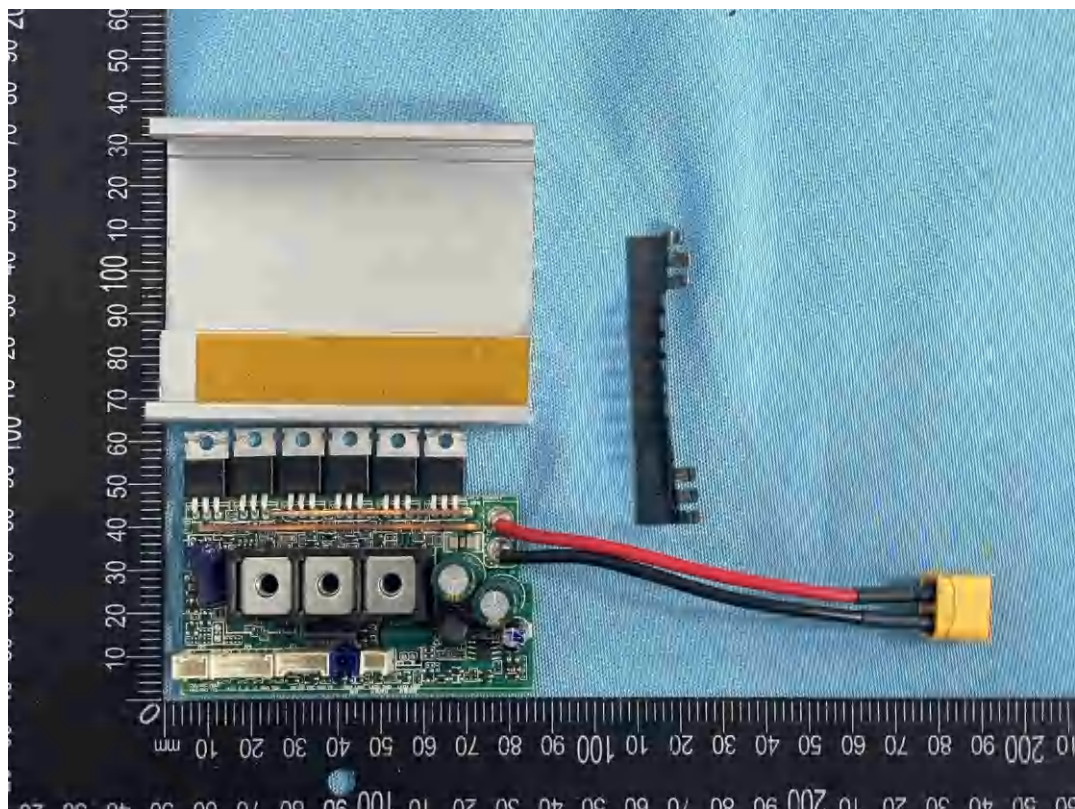
Figure 22: Controller view
