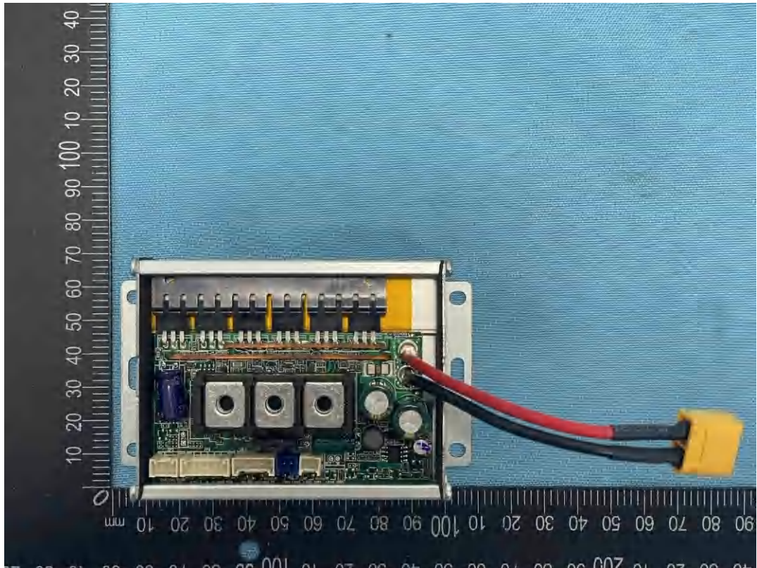
Figure 21: Controller view
