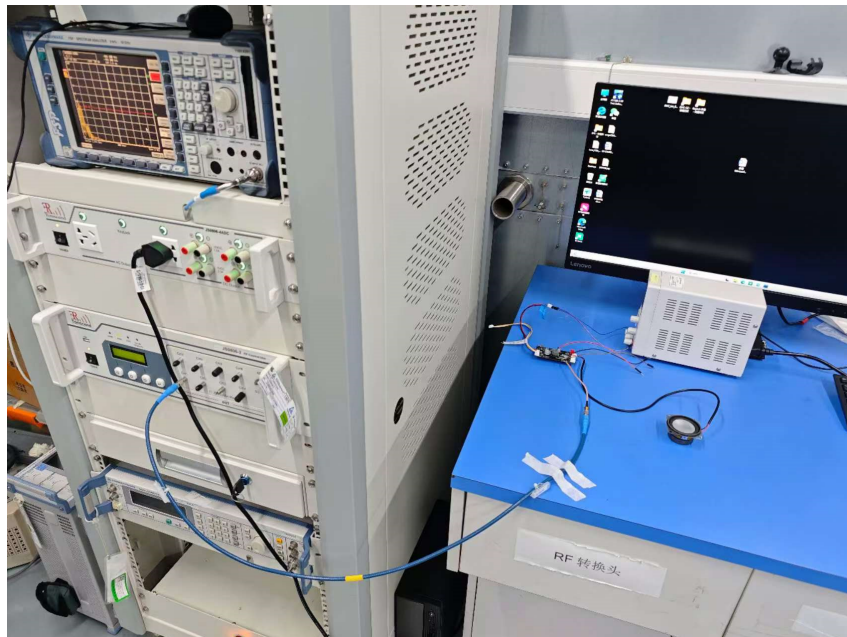
Photograph 1: Set-up photo for Conducted Emission
