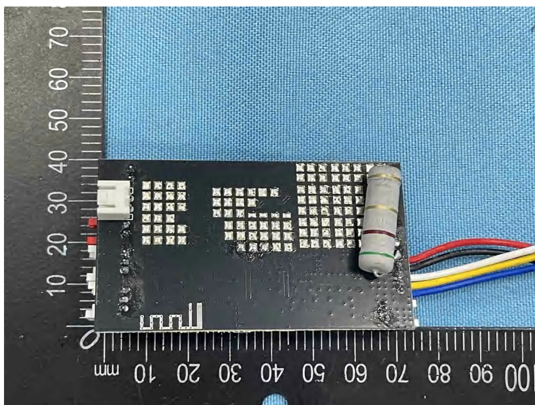
Figure 26: Internal view
