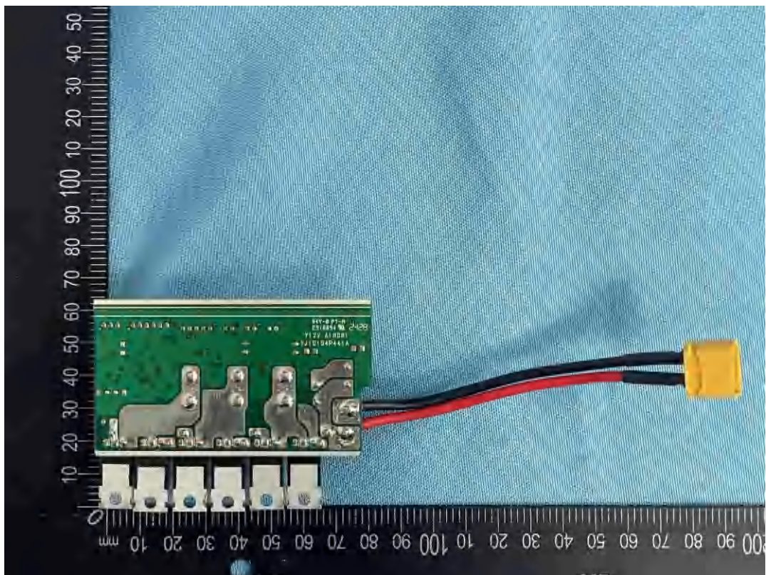
Figure 20: Controller PCB bottom view
