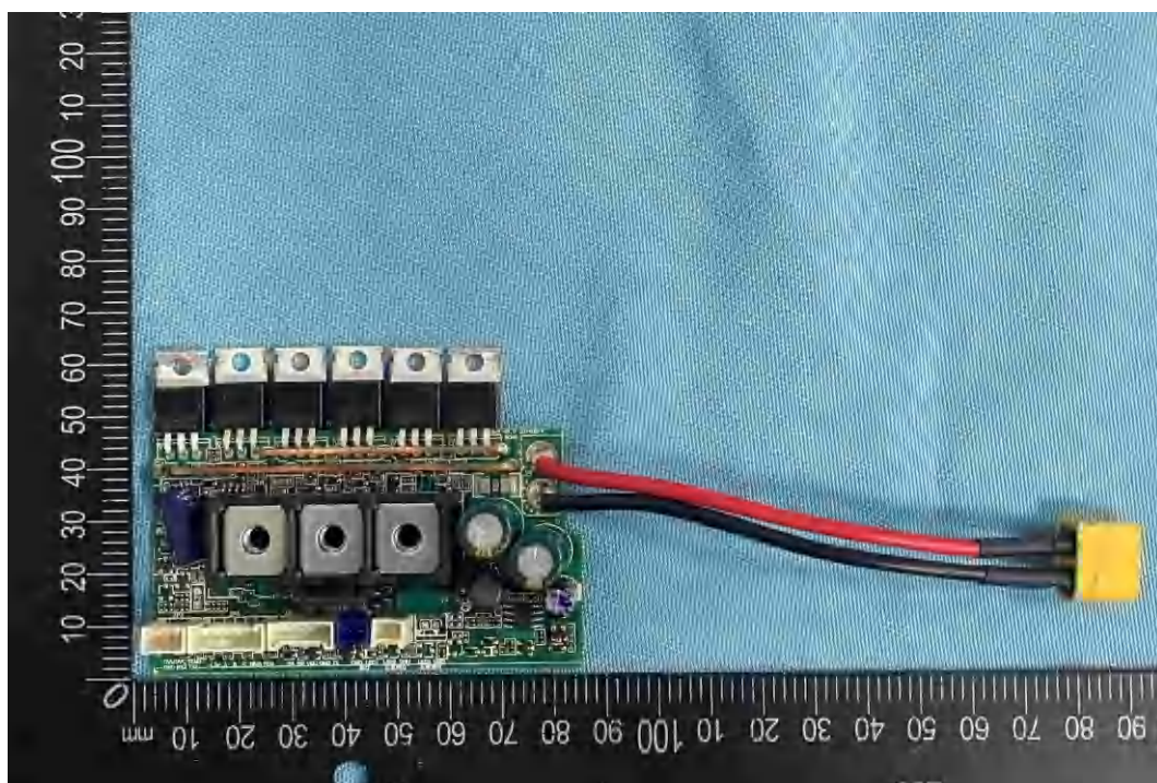
Figure 23: Controller PCB top view
