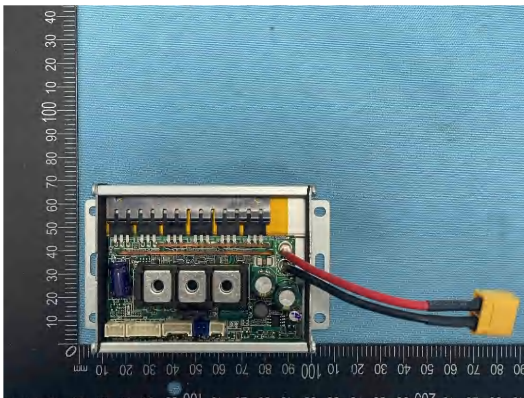
Figure 17: Controller view
