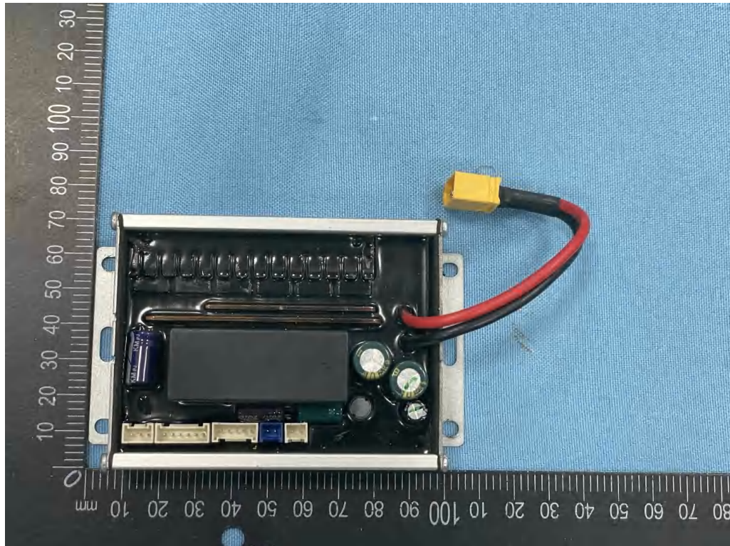
Figure 15: Controller view
