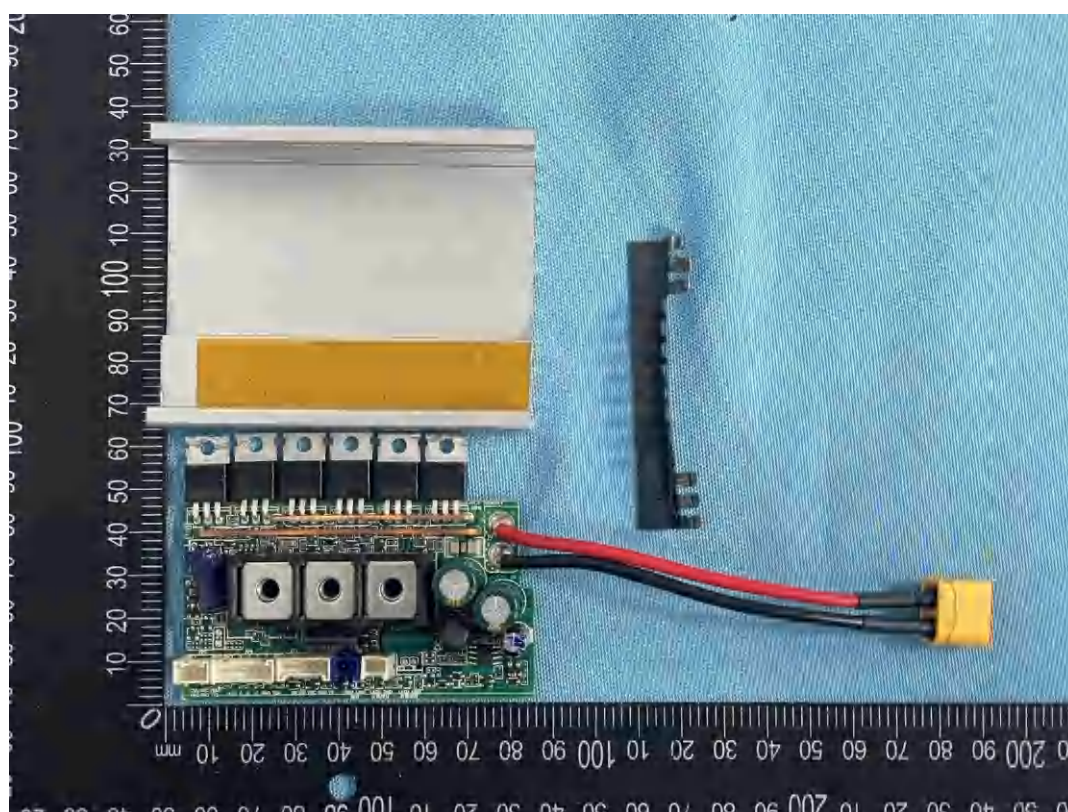
Figure 18: Controller view
