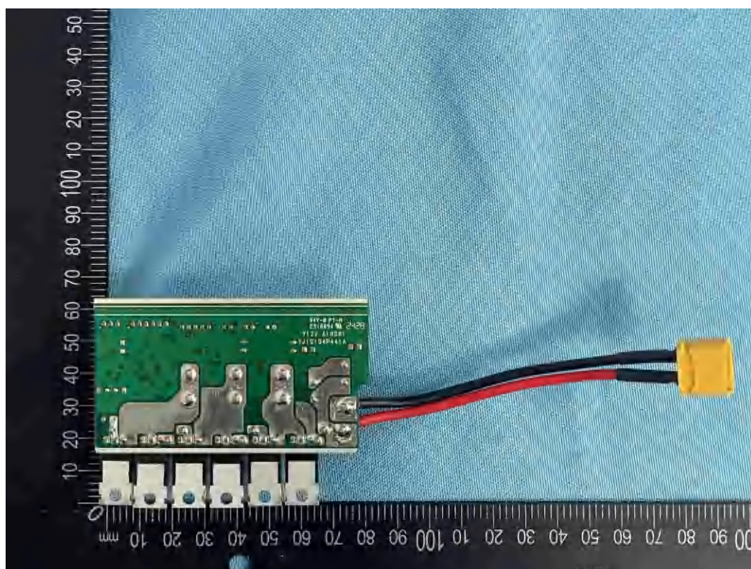
Figure 24: Controller PCB bottom view
