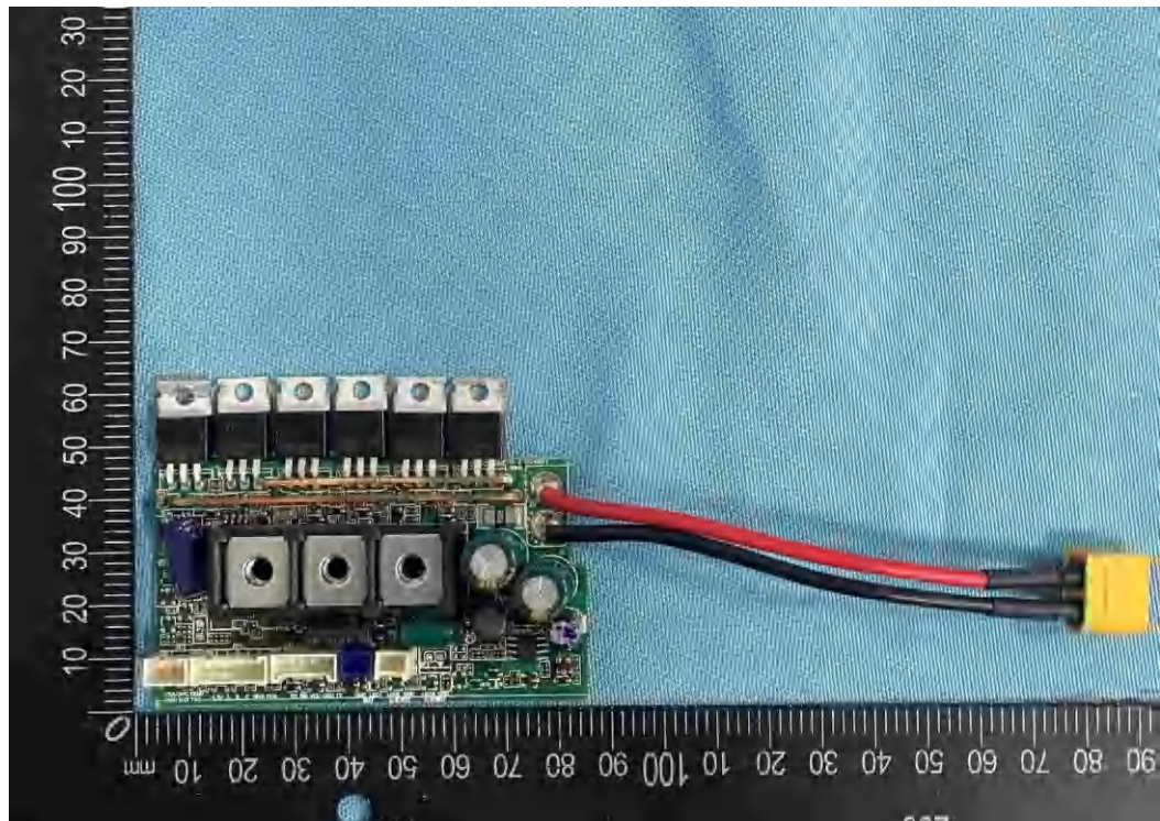
Figure 19: Controller PCB top view
