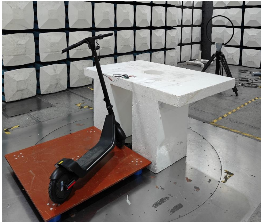
Photograph 1: Set-up photo for Radiated Spurious Emission, below 30MHz
