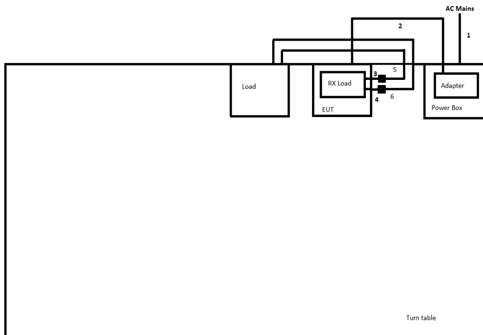
Test Setup Diagram – AC Line Conducted Emission Test – Mode 1 & 2
