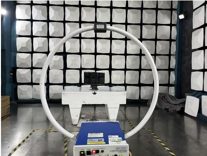
Radiated Test (9kHz-30MHz)
