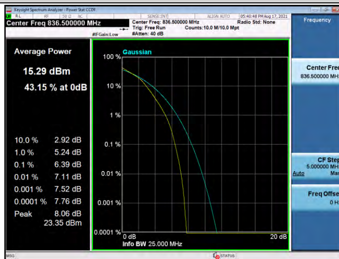
Band26-10MHz-16QAM-26990-50RB#0
