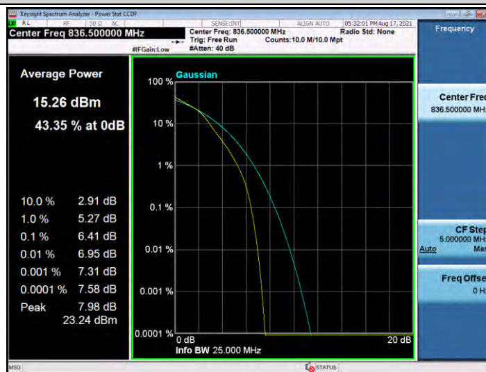
Band26-5MHz-16QAM-27015-25RB#0
