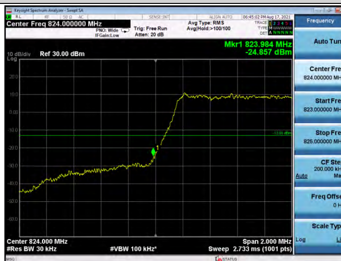
Band26-1.4MHz-16QAM-26797-6RB#0
