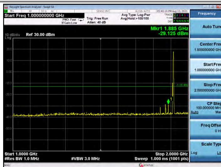
Band25-1.4MHz-QPSK-26683-1RB#0-Range3:2000~20000MHz
