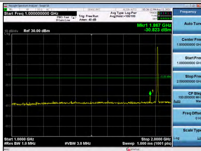
Band25-3MHz-QPSK-26675-1RB#0-Range3:2000~20000MHz
