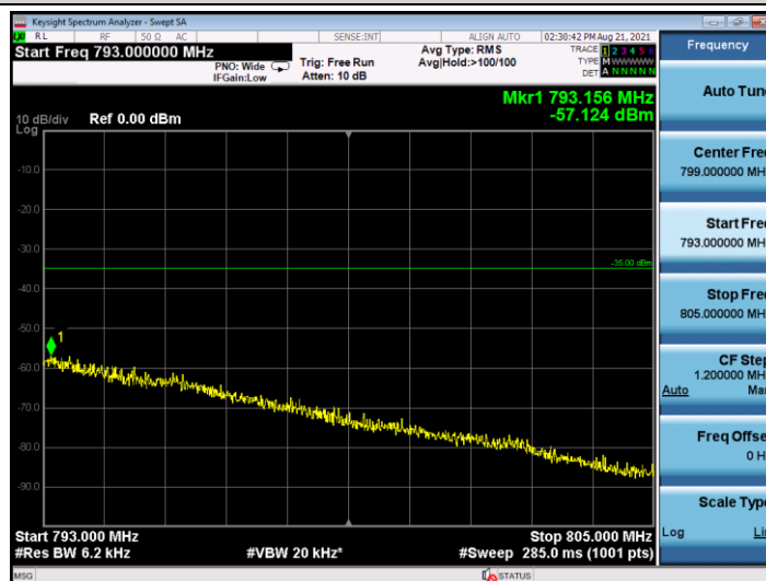
Band13-10MHz-16QAM-23230-50RB#0
