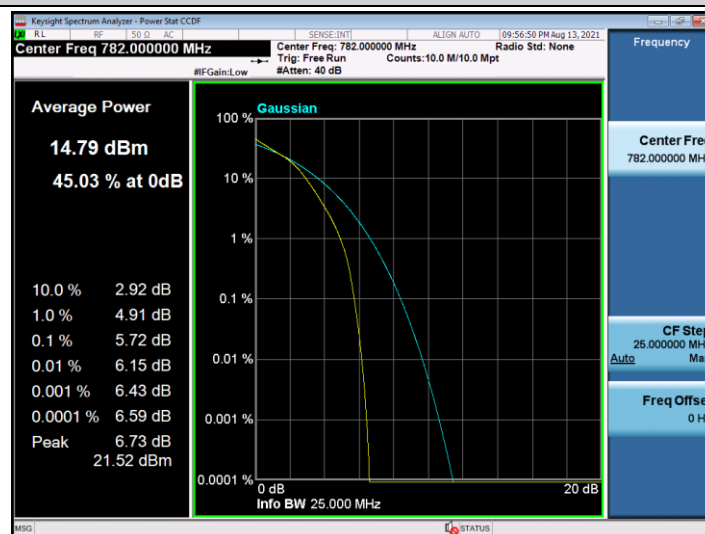
Band13-10MHz-16QAM-23230-50RB#0
