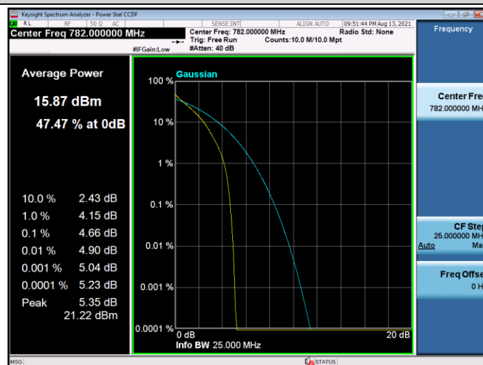
Band13-5MHz-QPSK-23255-25RB#0
