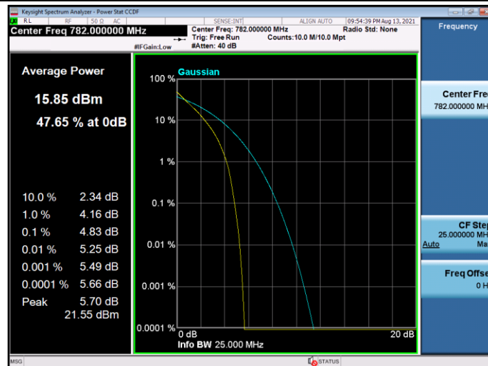
Band13-10MHz-16QAM-23230-50RB#0
