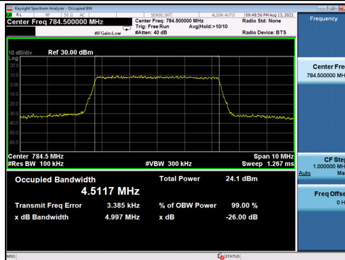
Band13-5MHz-16QAM-23205-25RB#0-4.505
