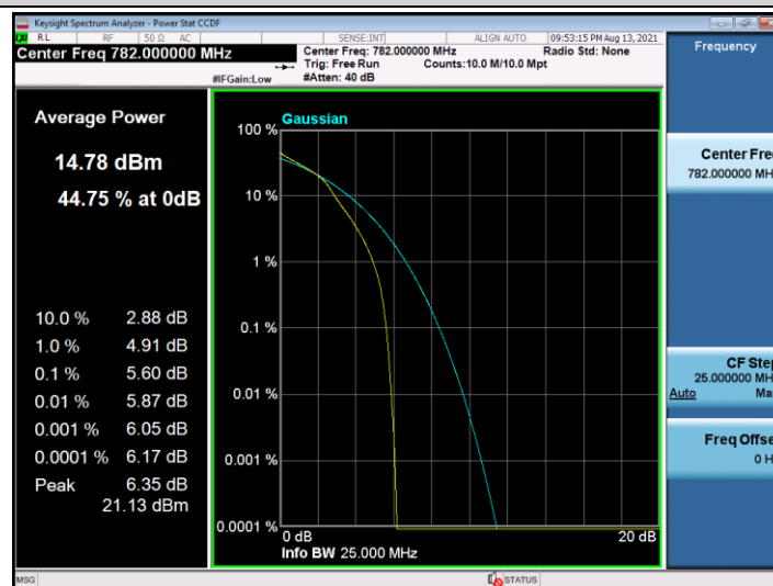
Band13-5MHz-16QAM-23255-25RB#0
