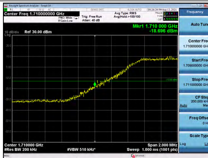
Band4-10MHz-QPSK-20350-50RB#0
