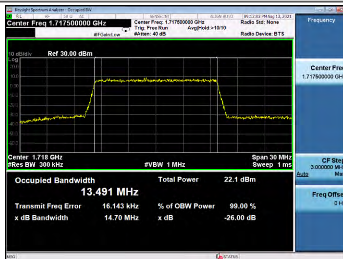
Band4-15MHz-16QAM-20175-75RB#0
