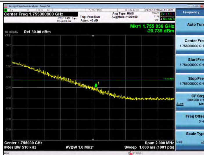
Band4-20MHz-16QAM-20300-100RB#0
