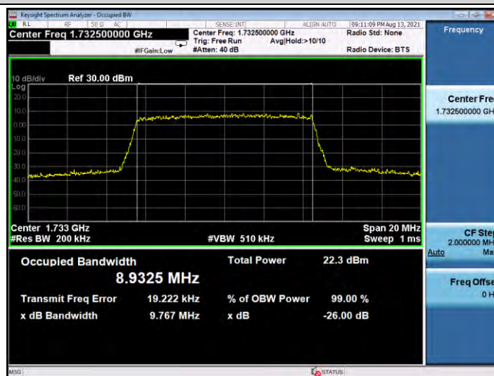
Band4-10MHz-16QAM-20350-50RB#0
