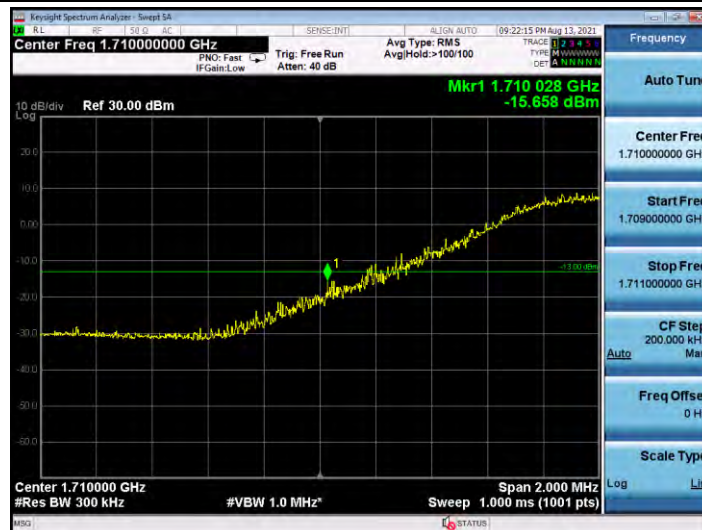
Band4-15MHz-QPSK-20325-75RB#0
