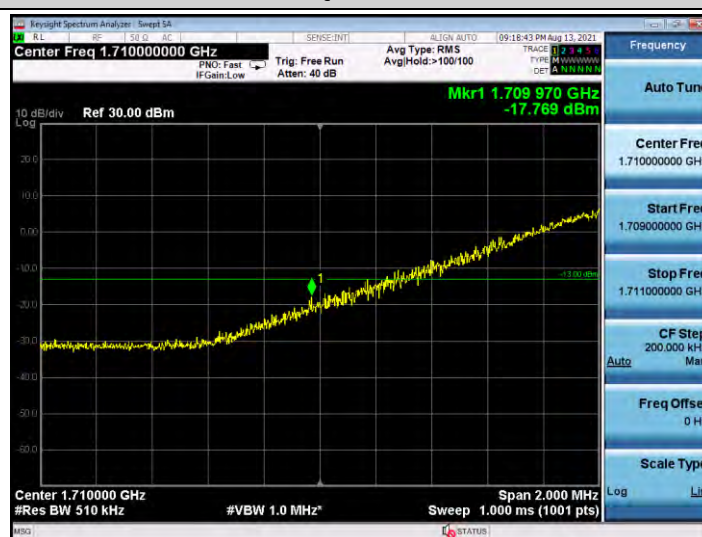
Band4-20MHz-QPSK-20300-100RB#0
