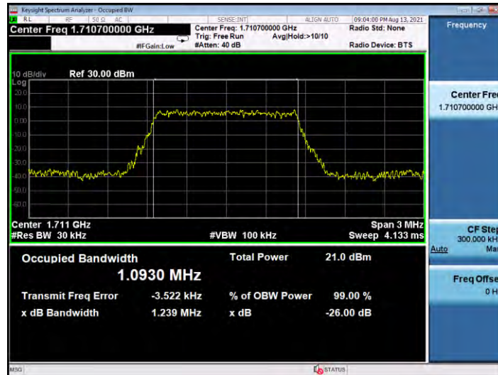
Band4-1.4MHz-QPSK-20175-6RB#0
