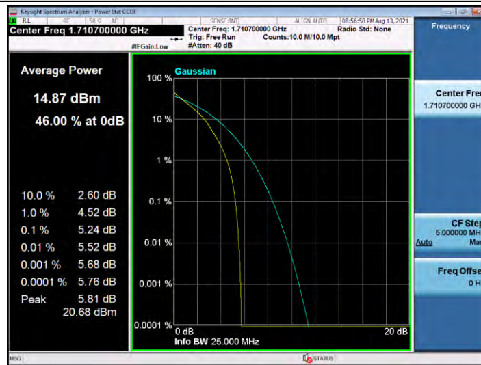
Band4-1.4MHz-QPSK-20175-6RB#0
