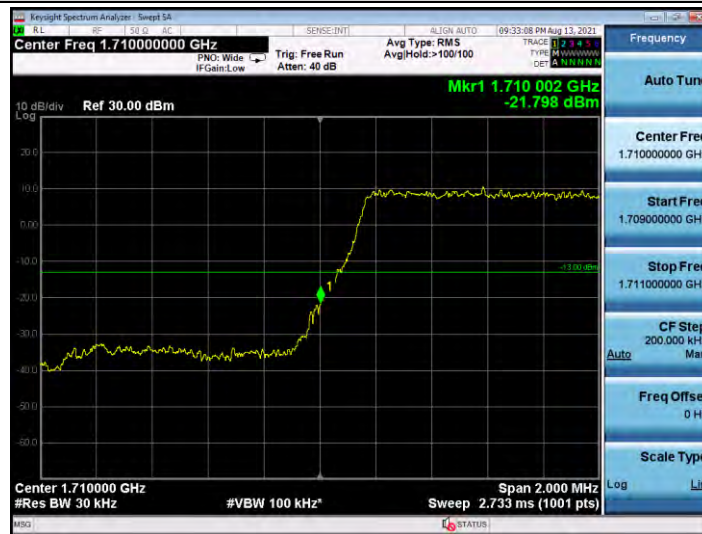
Band4-1.4MHz-QPSK-20393-6RB#0
