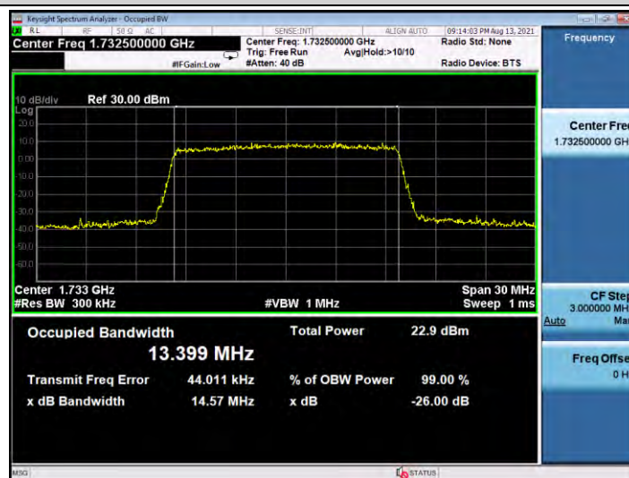
Band4-15MHz-QPSK-20325-75RB#0
