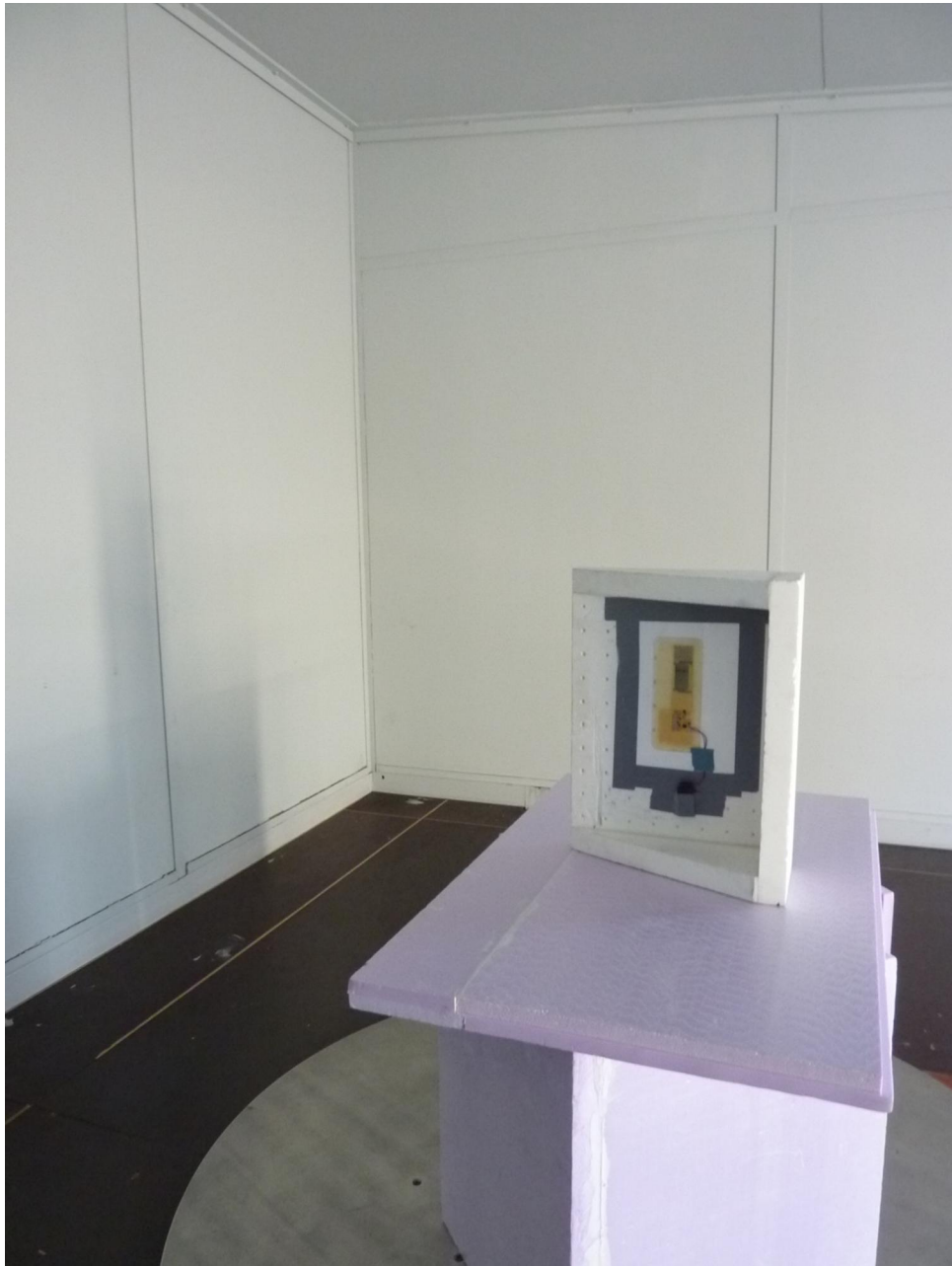
Test setup open area test site 9 kHz – 1 GHz
