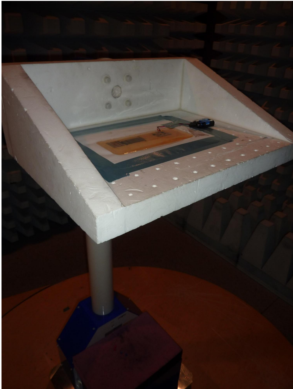
Test setup CET214 - Test setup fully anechoic chamber
