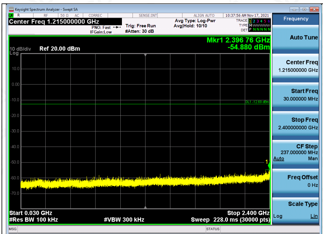
Test_Graph_802.11b_ANT1_2437_11Mbps_Lower Band Emissions
