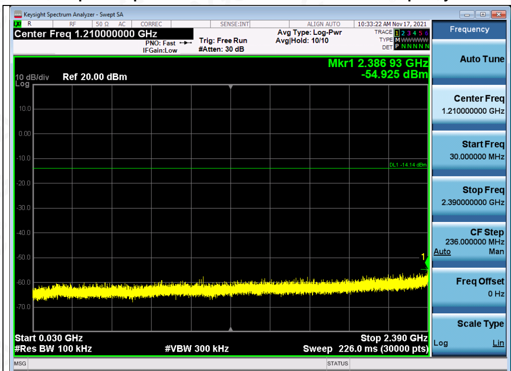
Test_Graph_802.11b_ANT1_2412_11Mbps_Lower Band Emissions
