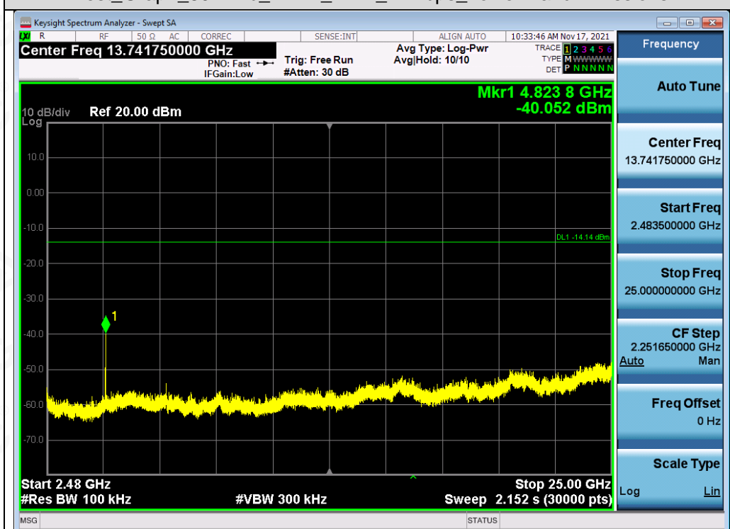
Test_Graph_802.11b_ANT1_2412_11Mbps_Higher Band Emissions
