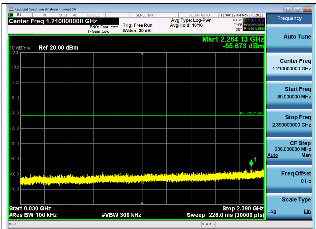
Test_Graph_802.11g_ANT1_2412_54Mbps_Lower Band Emissions
