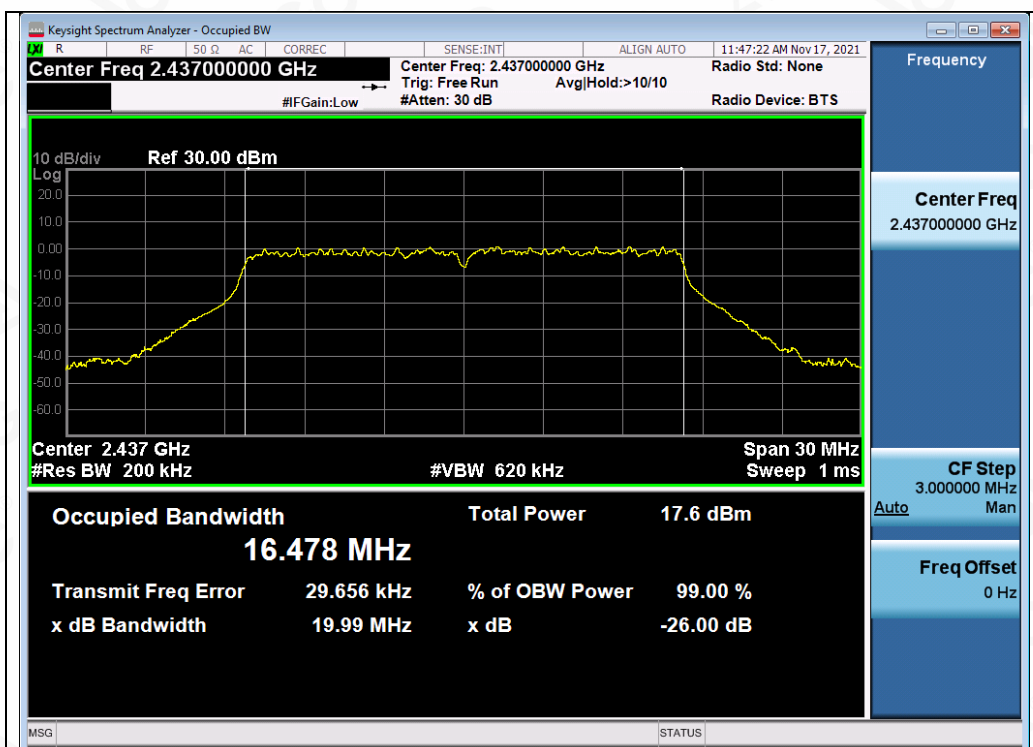
Test_Graph_802.11g_ANT1_2437_54Mbps_OBW
