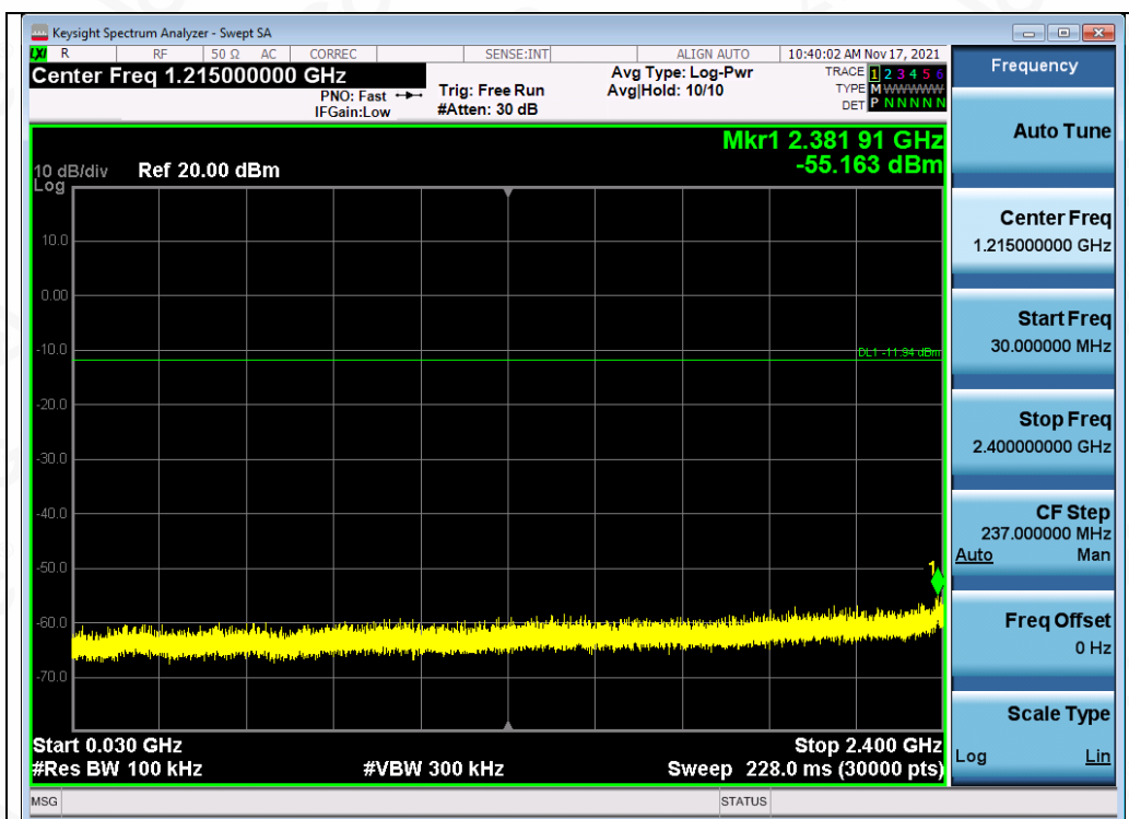
Test_Graph_802.11b_ANT1_2462_11Mbps_Lower Band Emissions
