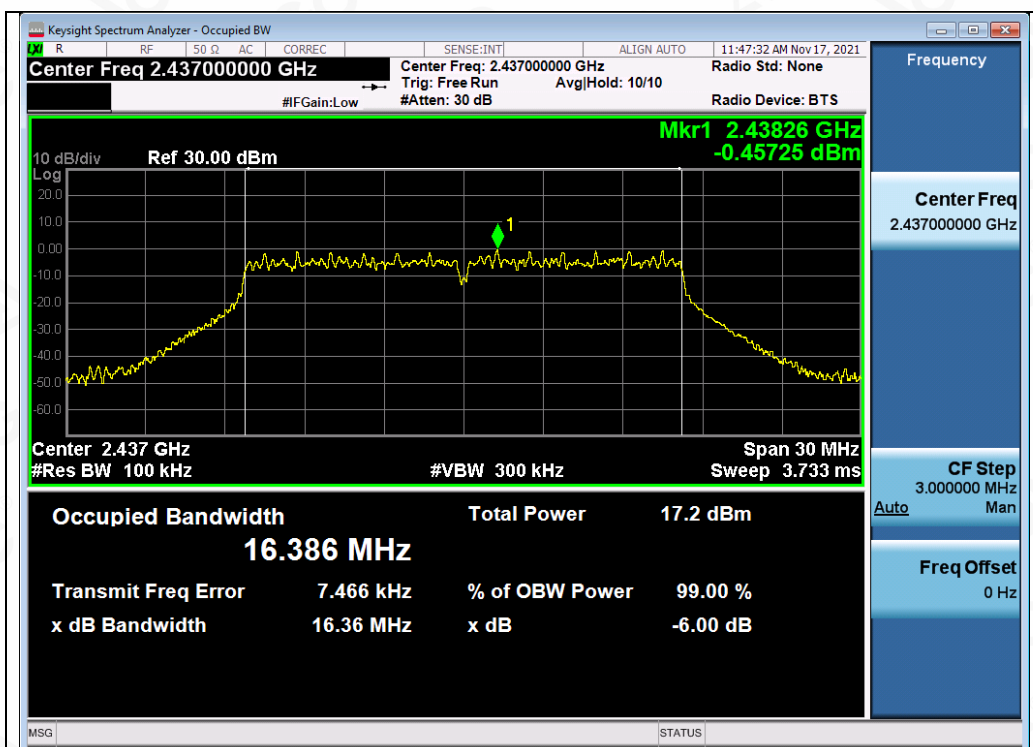
Test_Graph_802.11g_ANT1_2437_54Mbps_DTSBW
