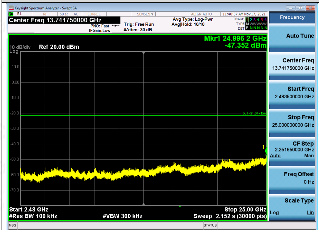
Test_Graph_802.11g_ANT1_2412_54Mbps_Higher Band Emissions
