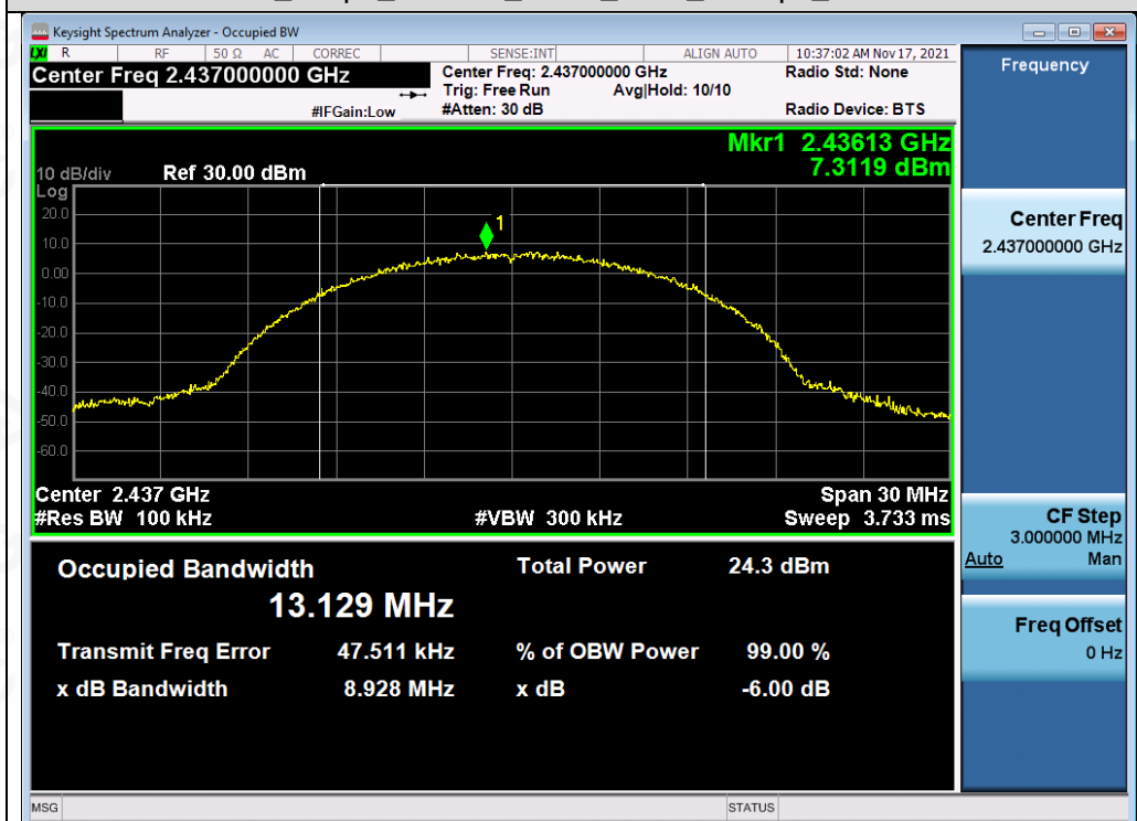
Test_Graph_802.11b_ANT1_2437_11Mbps_DTSBW
