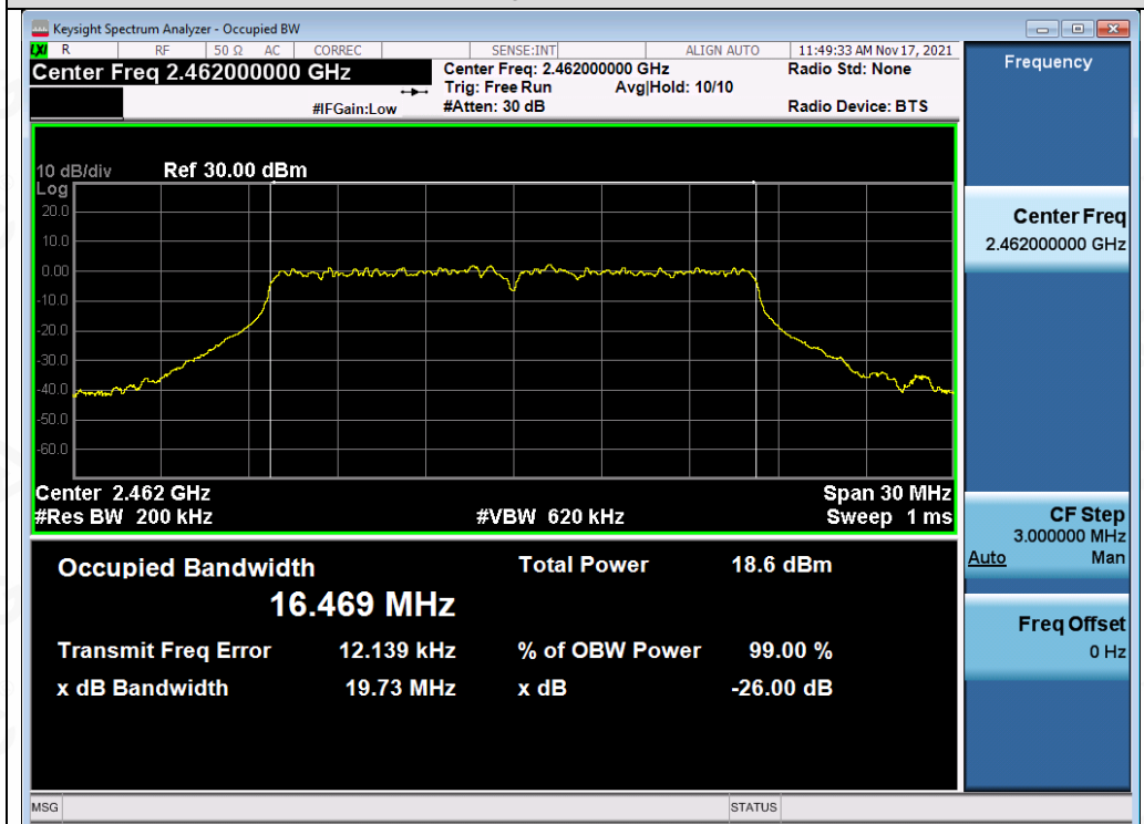
Test_Graph_802.11g_ANT1_2462_54Mbps_OBW
