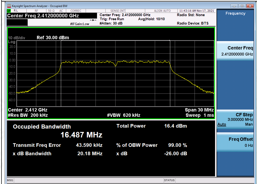
Test_Graph_802.11g_ANT1_2412_54Mbps_OBW
