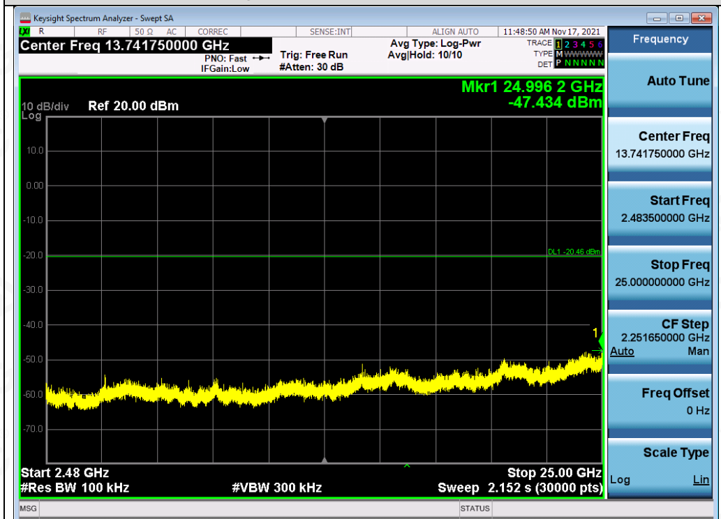
Test_Graph_802.11g_ANT1_2437_54Mbps_Higher Band Emissions
