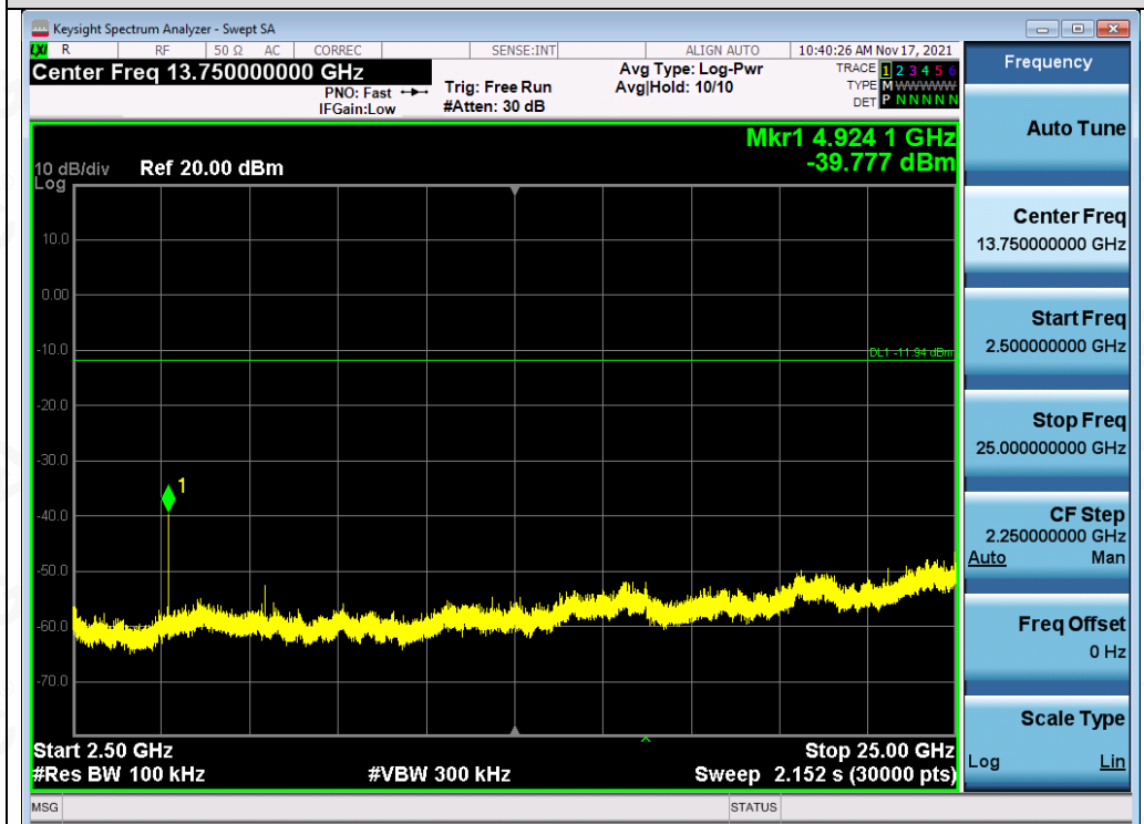
Test_Graph_802.11b_ANT1_2462_11Mbps_Higher Band Emissions
