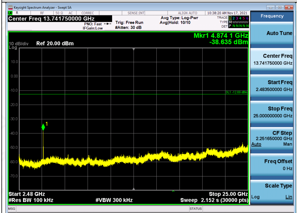
Test_Graph_802.11b_ANT1_2437_11Mbps_Higher Band Emissions
