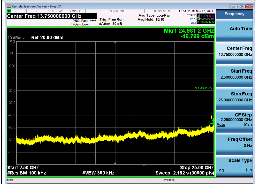
Test_Graph_802.11g_ANT1_2462_54Mbps_Higher Band Emissions
