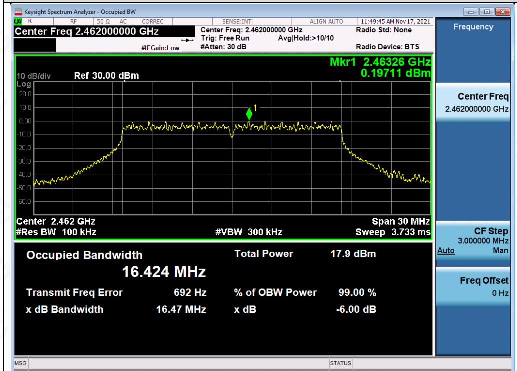
Test_Graph_802.11g_ANT1_2462_54Mbps_DTSBW
