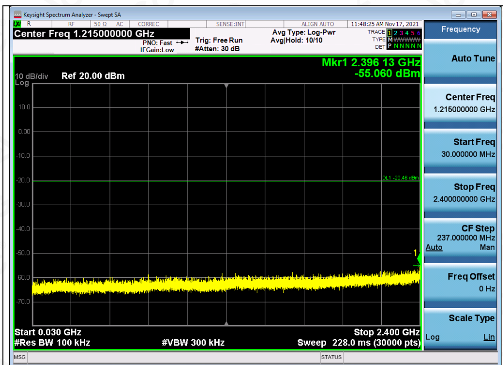
Test_Graph_802.11g_ANT1_2437_54Mbps_Lower Band Emissions
