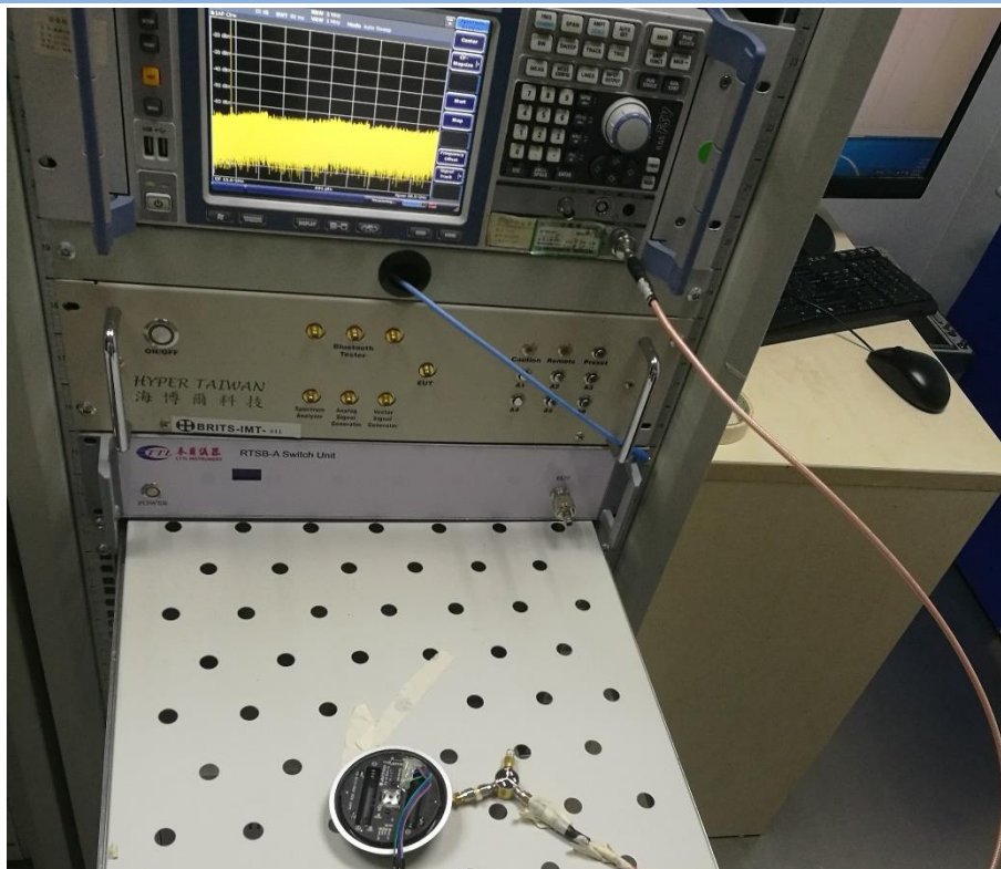
Conducted Test-BLE
