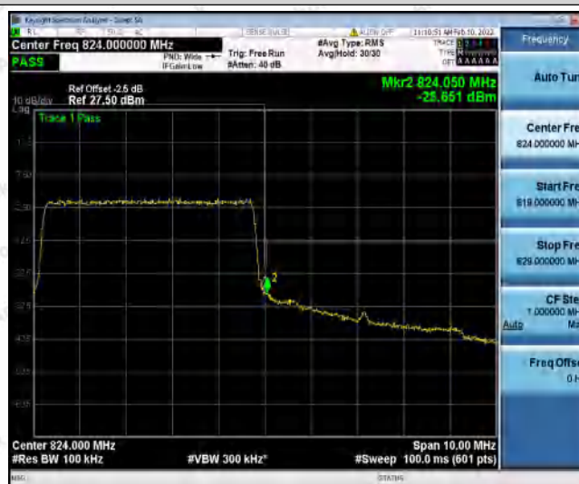
Band26-5MHz-QPSK-26815-1RB#0
