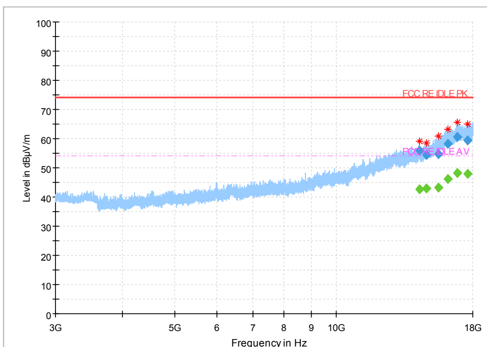
Fig.47 Radiated Spurious Emission (802.11b,Ch11,3GHz~18GHz)
