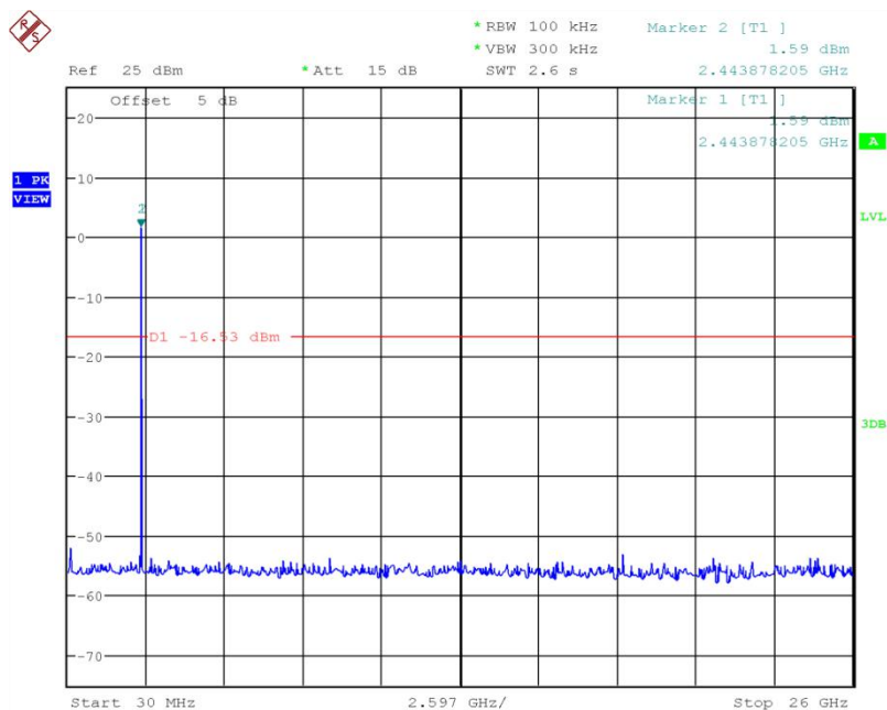
Fig.29 Conducted Spurious Emission (802.11b, Ch11)
