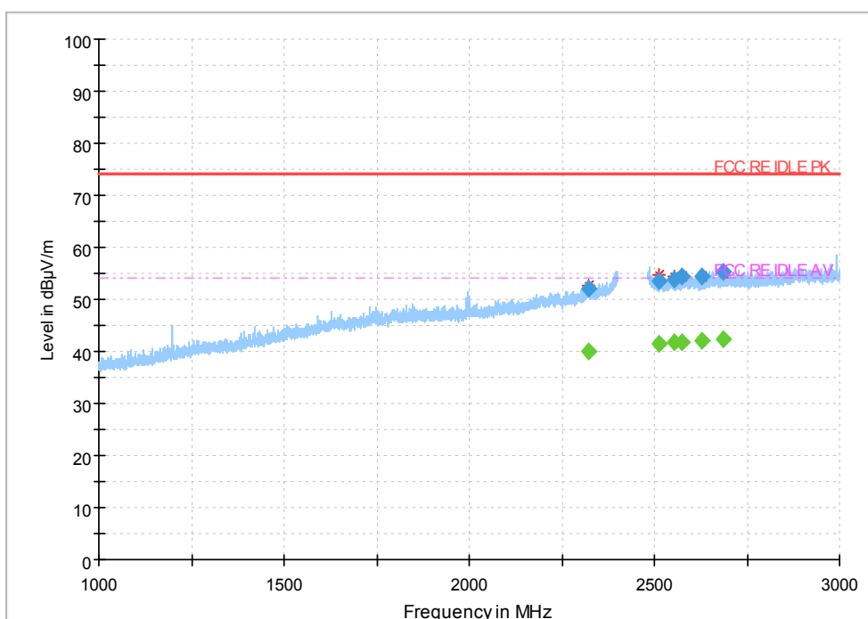
Fig.22 Radiated emission: Ch39, 1GHz~3GHz
