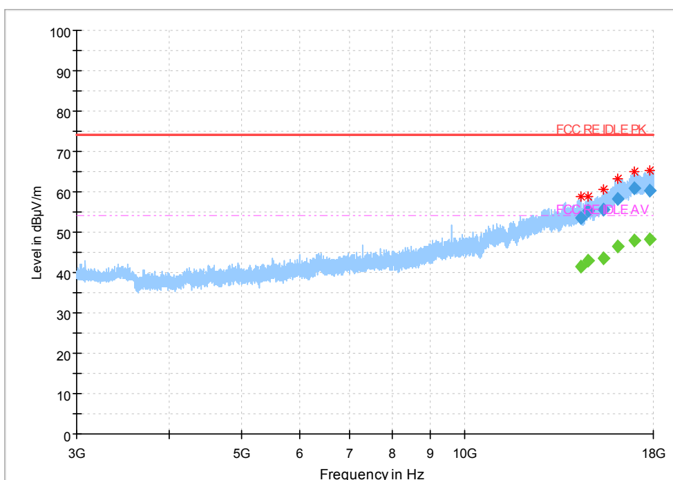
Fig.20 Radiated emission: Ch0, 3GHz~18GHz
