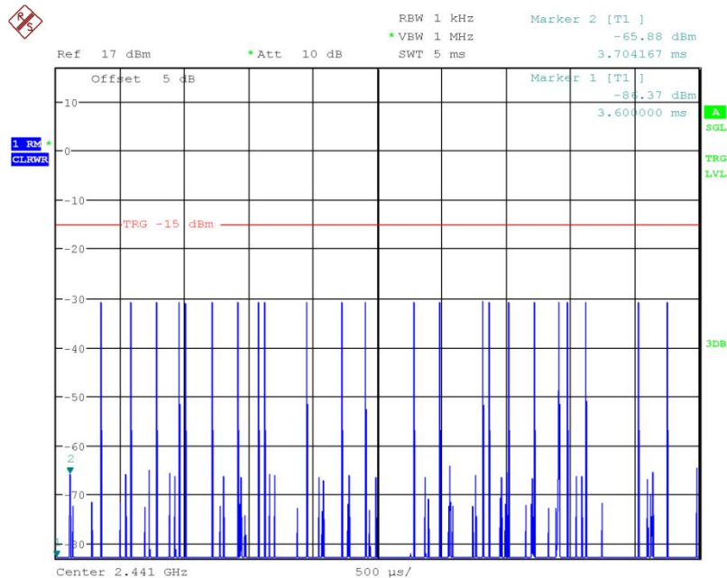
Fig.70 Number of Transmissions Measurement: Ch39, Packet 3-DH3
