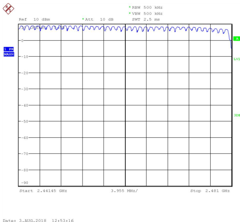
Fig.90 Number of hopping frequency: 8DPSK, Ch40~78
