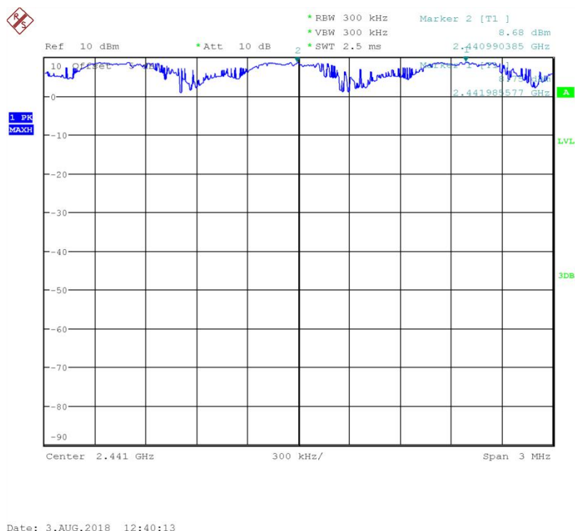
Fig.84 Carrier separation measurement: 8DPSK, Ch39
