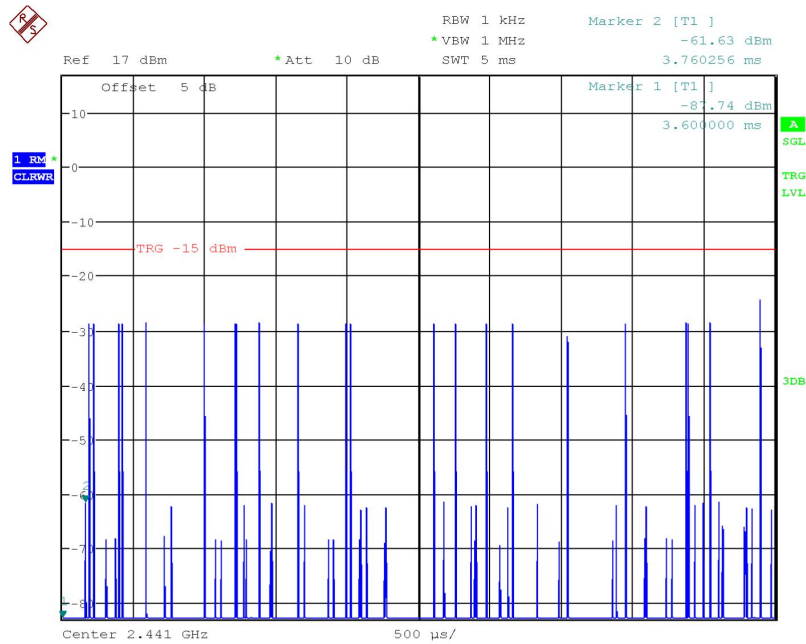
Fig.64 Number of Transmissions Measurement: Ch39, Packet 2-DH3
