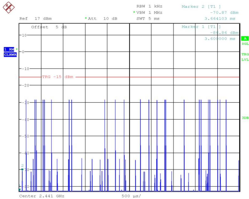
Fig.68 Number of Transmissions Measurement: Ch39, Packet 3-DH1
