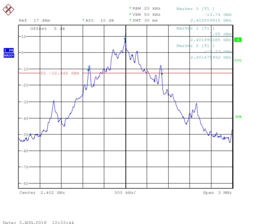
Fig.73 20dB Bandwidth: GFSK, Ch0
