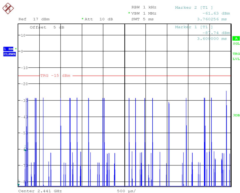
Fig.62 Number of Transmissions Measurement: Ch39, Packet 2-DH1
