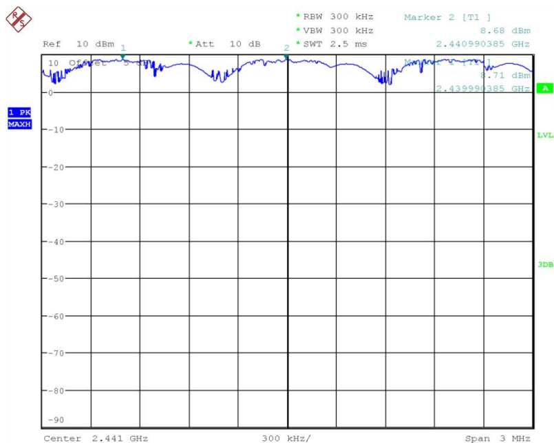
Fig.82 Carrier separation measurement: GFSK, Ch39
