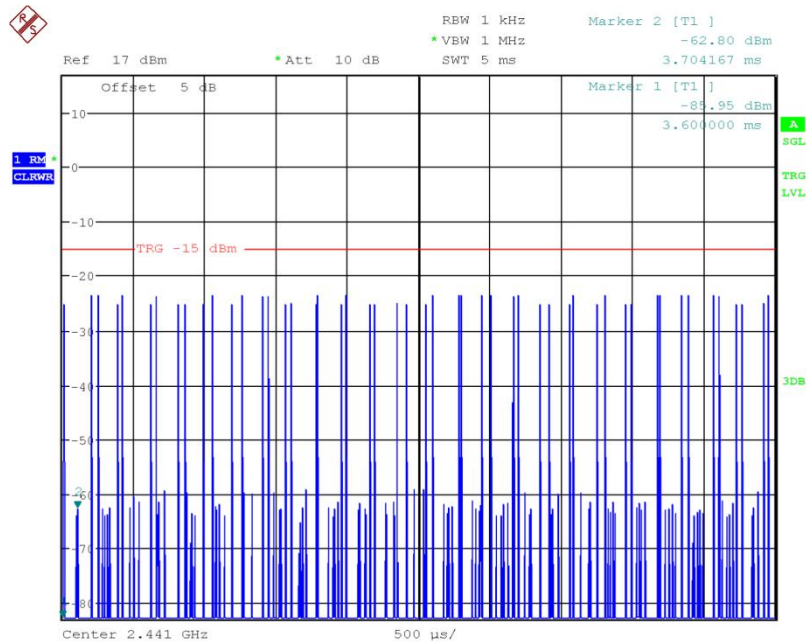
Fig.56 Number of Transmissions Measurement: Ch39, Packet DH1
