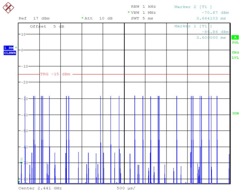
Fig.66 Number of Transmissions Measurement: Ch39, Packet 2-DH5
