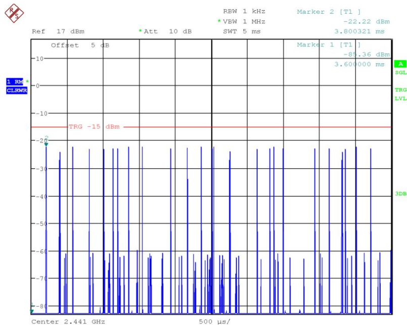
Fig.58 Number of Transmissions Measurement: Ch39, Packet DH3
