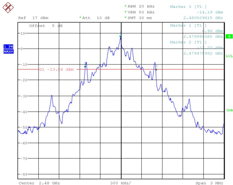
Fig.74 20dB Bandwidth: GFSK, Ch39
