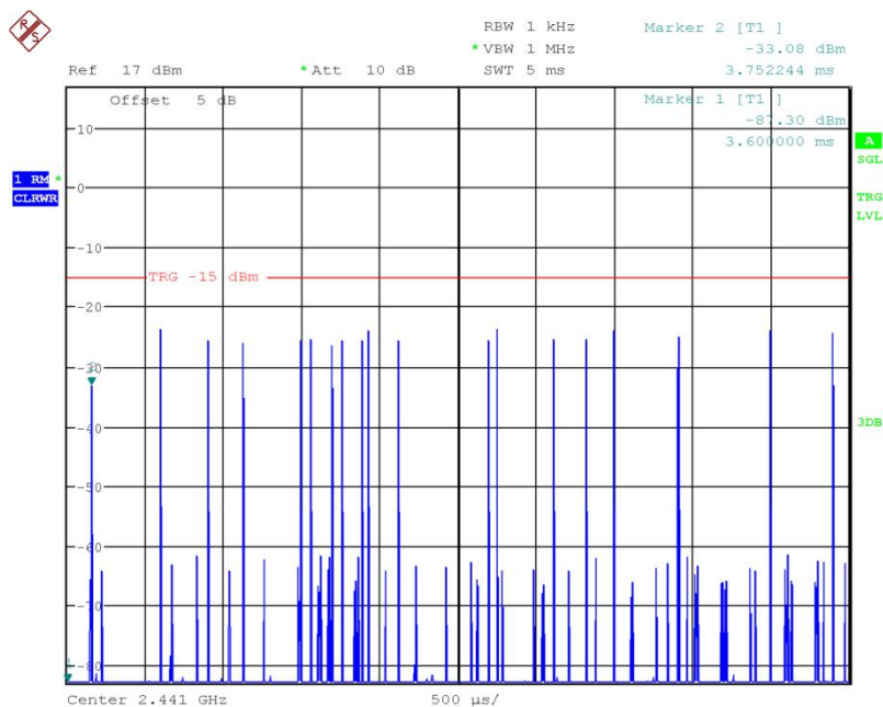
Fig.60 Number of Transmissions Measurement: Ch39, Packet DH5
