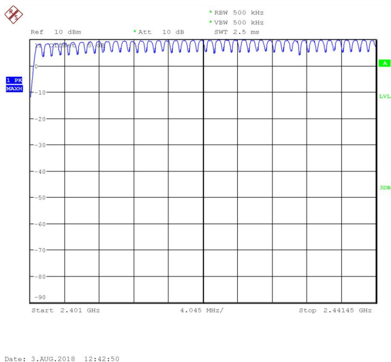
Fig.85 Number of hopping frequency: GFSK, Ch0~39
