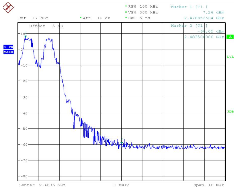
Fig.20 Frequency Band Edge: 8DPSK, Ch78, Hopping OFF
