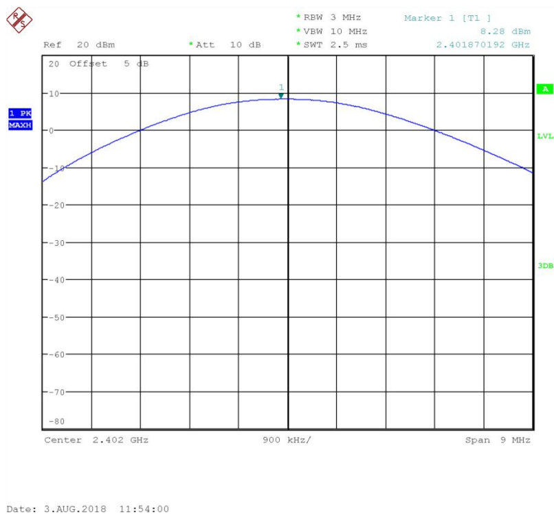
Fig.1 Peak Conducted Output Power CH0, DH1
