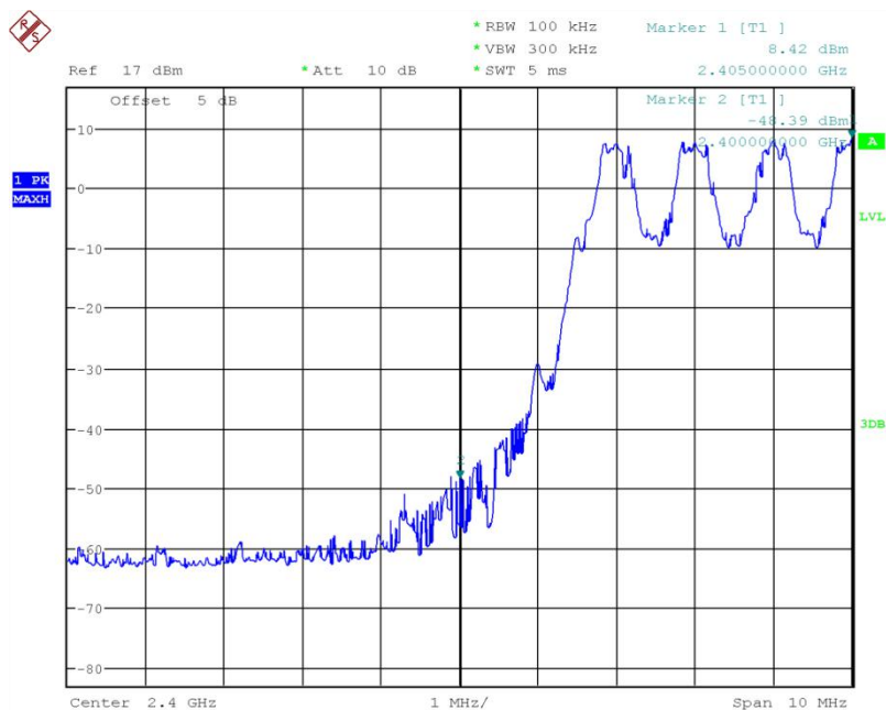
Fig.18 Frequency Band Edge: 8DPSK, Ch0, Hopping OFF
