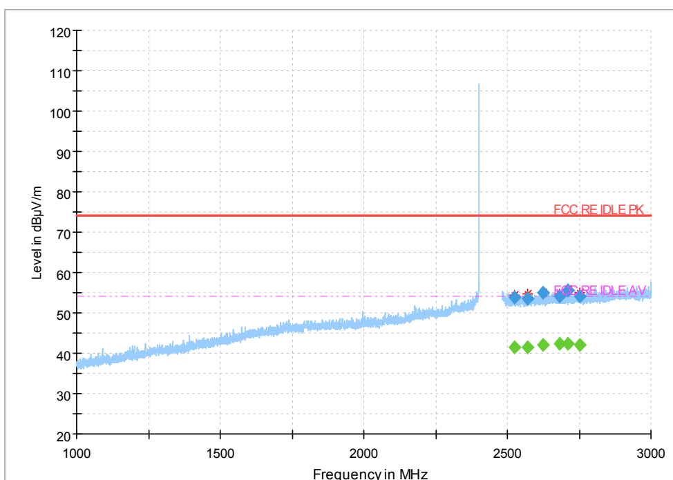
Fig.41 Radiated emission: GFSK, Ch0, 1GHz~3GHz
