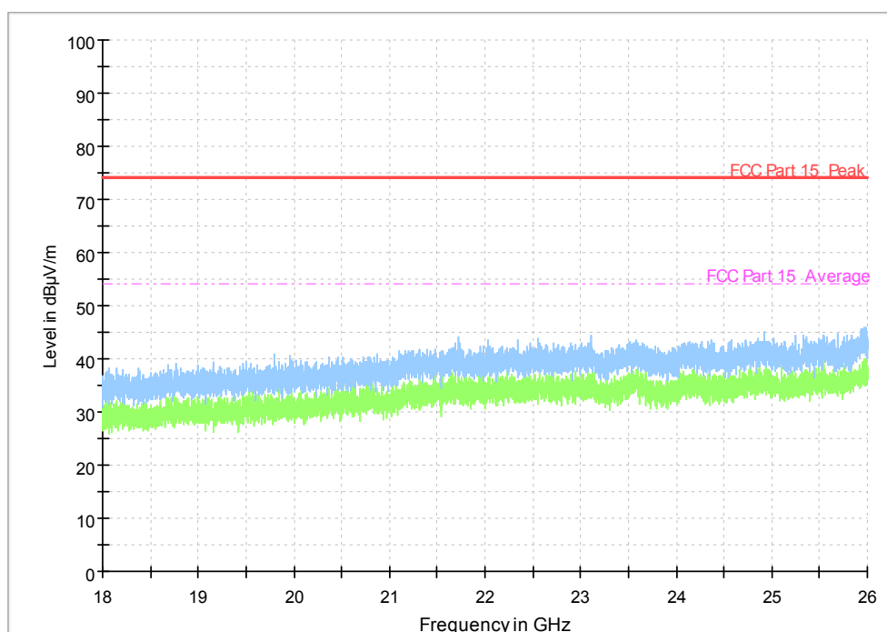
Fig.54 Radiated emission (Power): 8DPSK, high channel
