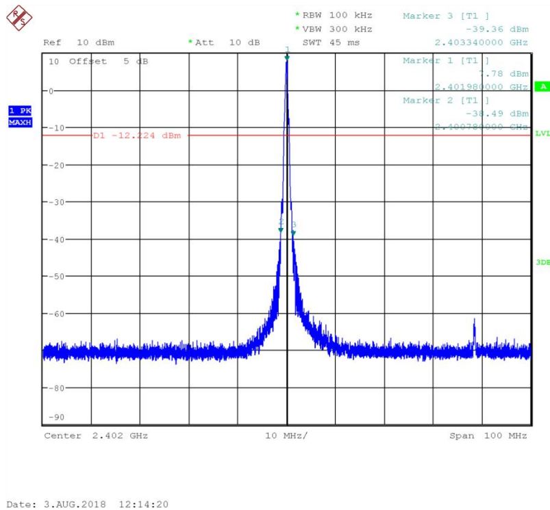
Fig.22 Conducted spurious emission: GFSK, Ch0, 2402MHz
