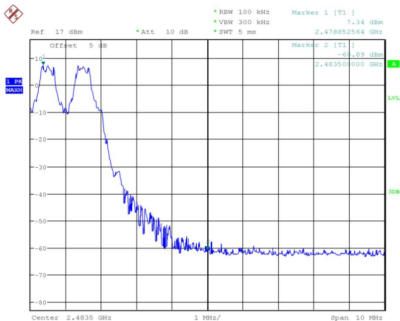
Fig.12 Frequency Band Edge: GFSK, Ch78, Hopping OFF
