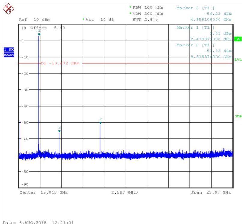
Fig.39 Conducted spurious emission: 8DPSK, Ch78, 30MHz~26GHz
